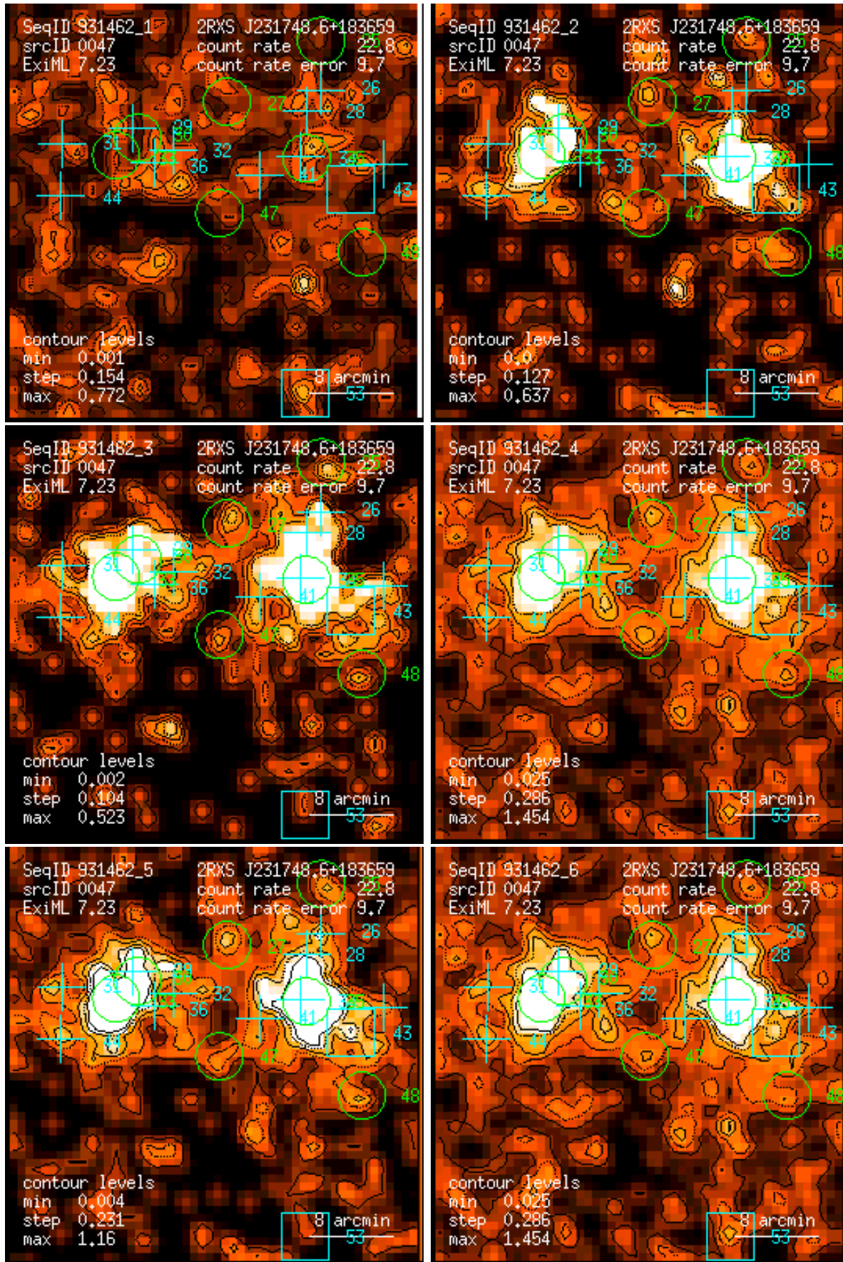
Figure 47: RASS 931462: detection 0047: band rate images, Gaussian filter: (1) PSPC channels 11 – 41, (2) 52 – 90, (3) 91 – 201, (4) 11 – 235, (5) 52 – 201, (6) 11 – 201. Broad band rates in counts/ks. Band rate contour levels in counts/ks/arcmin 2 .
