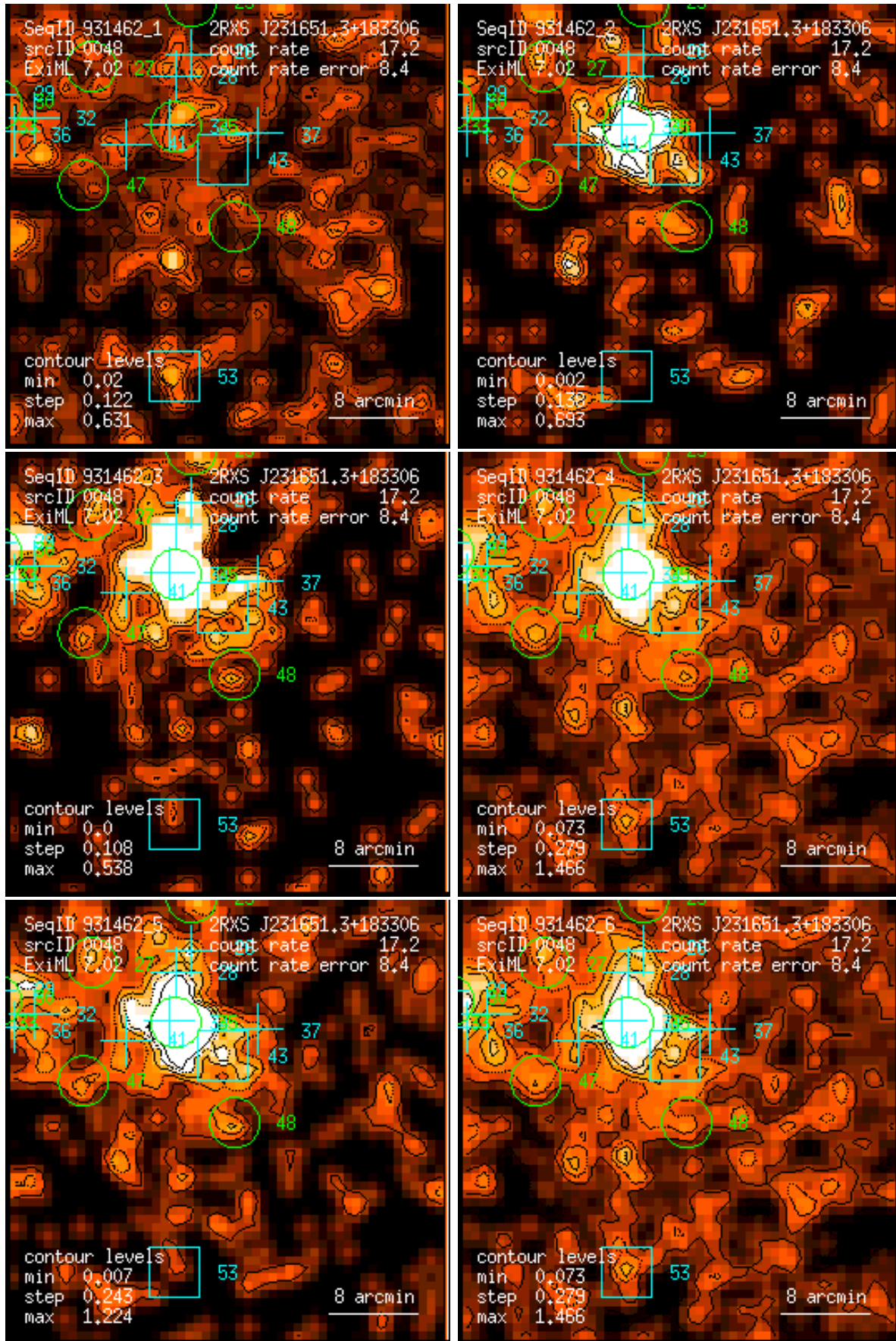
Figure 48: RASS 931462: detection 0048: band rate images, Gaussian filter: (1) PSPC channels 11 – 41, (2) 52 – 90, (3) 91 – 201, (4) 11 – 235, (5) 52 – 201, (6) 11 – 201. Broad band rates in counts/ks. Band rate contour levels in counts/ks/arcmin 2 .
