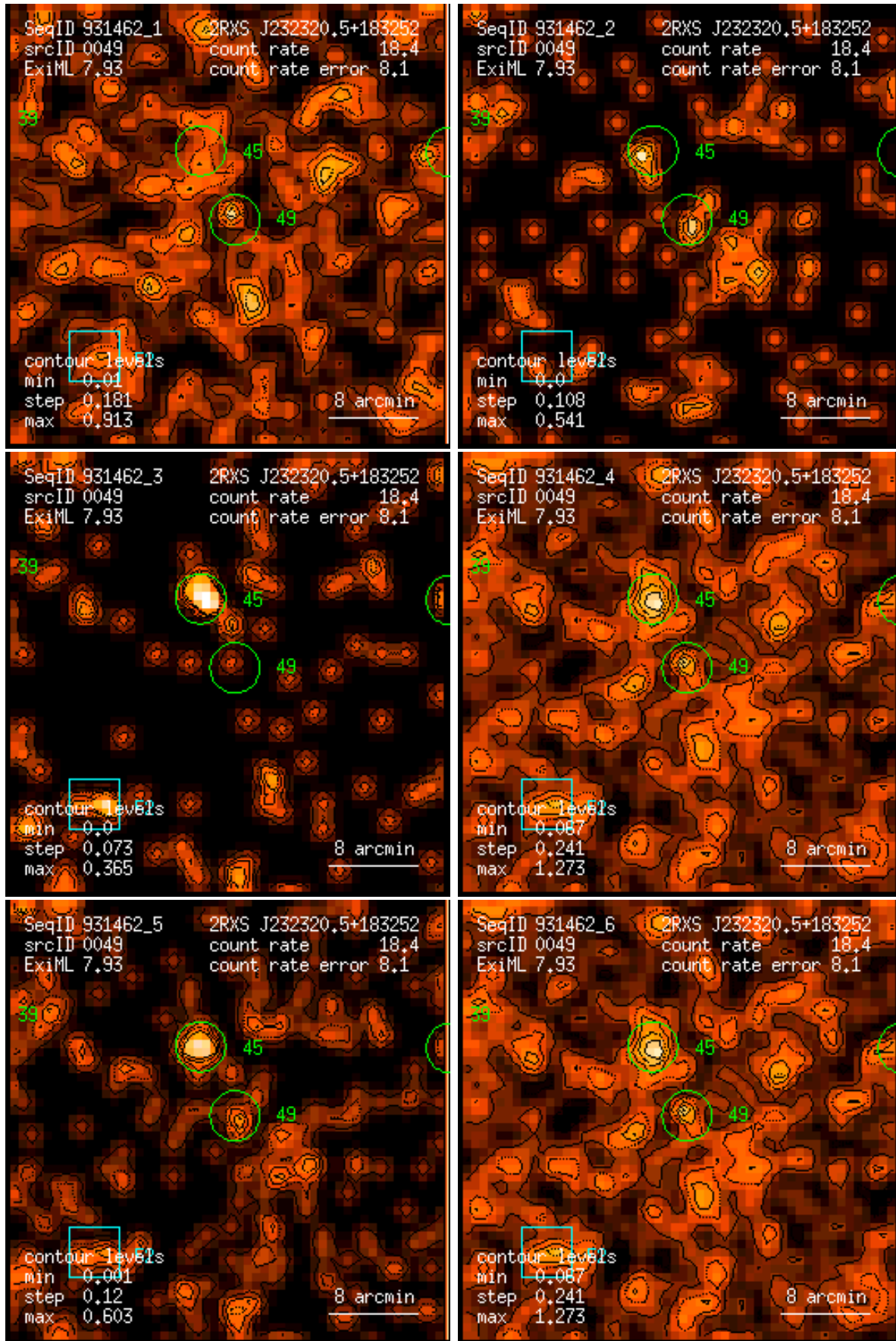
Figure 49: RASS 931462: detection 0049: band rate images, Gaussian filter: (1) PSPC channels 11 – 41, (2) 52 – 90, (3) 91 – 201, (4) 11 – 235, (5) 52 – 201, (6) 11 – 201. Broad band rates in counts/ks. Band rate contour levels in counts/ks/arcmin 2 .
