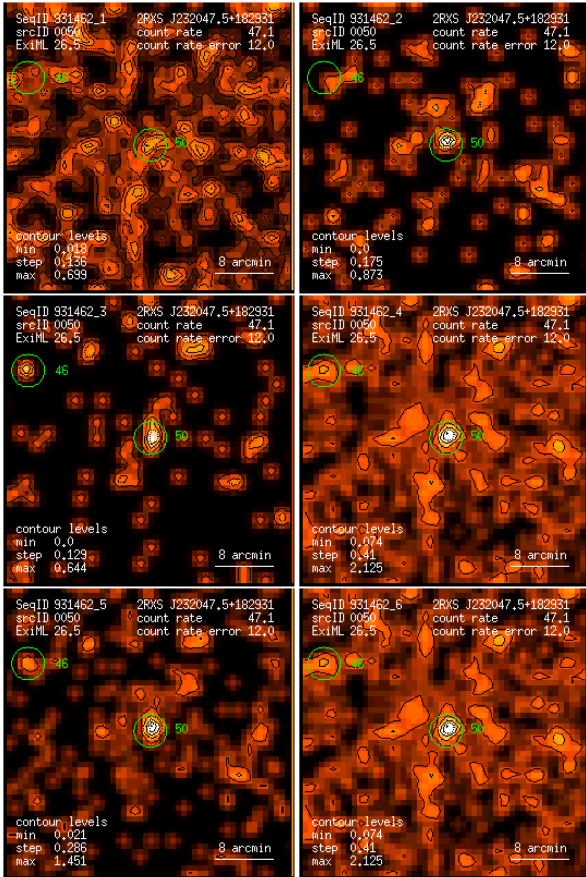
Figure 50: RASS 931462: detection 0050: band rate images, Gaussian filter: (1) PSPC channels 11 – 41, (2) 52 – 90, (3) 91 – 201, (4) 11 – 235, (5) 52 – 201, (6) 11 – 201. Broad band rates in counts/ks. Band rate contour levels in counts/ks/arcmin 2 .
