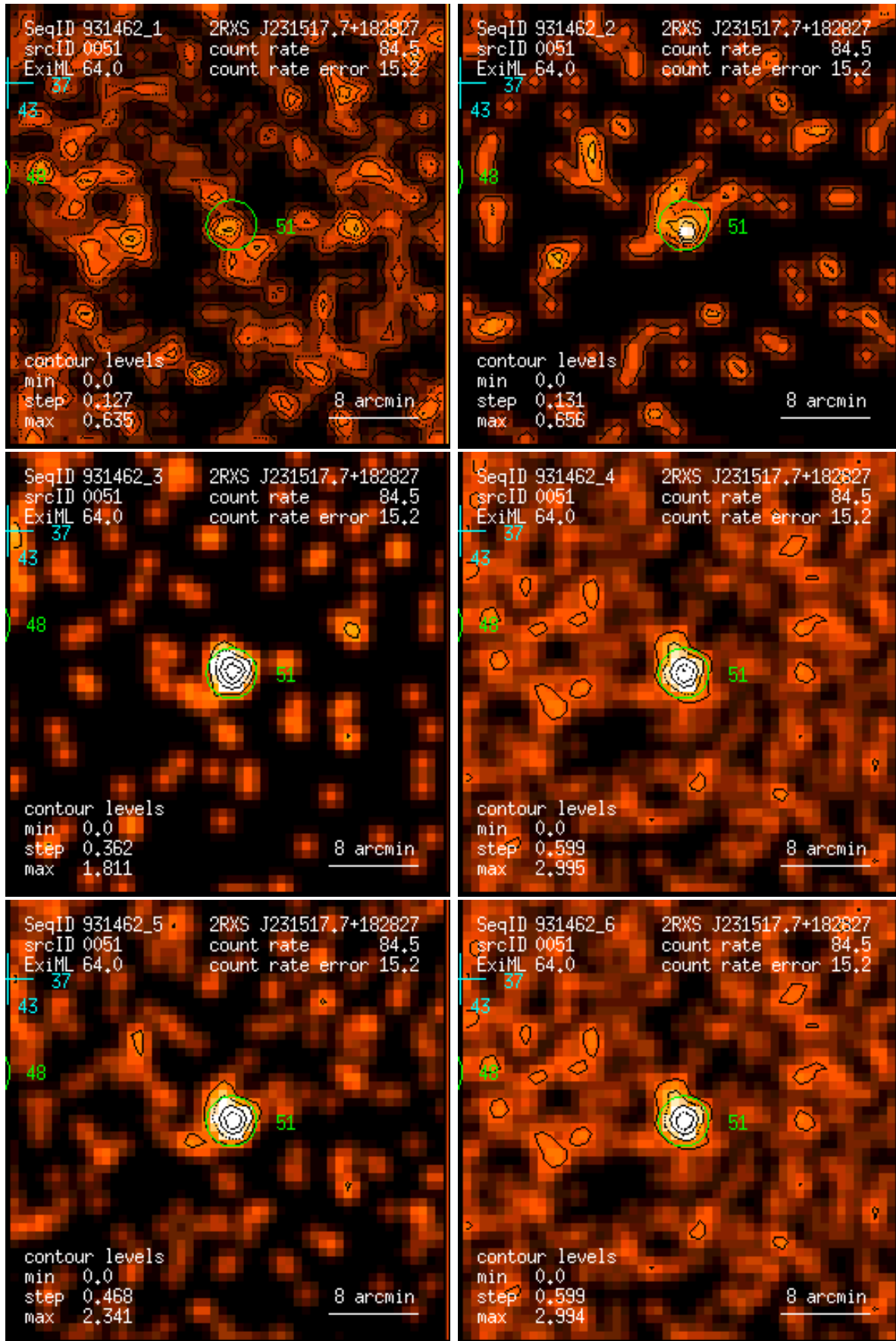
Figure 51: RASS 931462: detection 0051: band rate images, Gaussian filter: (1) PSPC channels 11 – 41, (2) 52 – 90, (3) 91 – 201, (4) 11 – 235, (5) 52 – 201, (6) 11 – 201. Broad band rates in counts/ks. Band rate contour levels in counts/ks/arcmin 2 .
