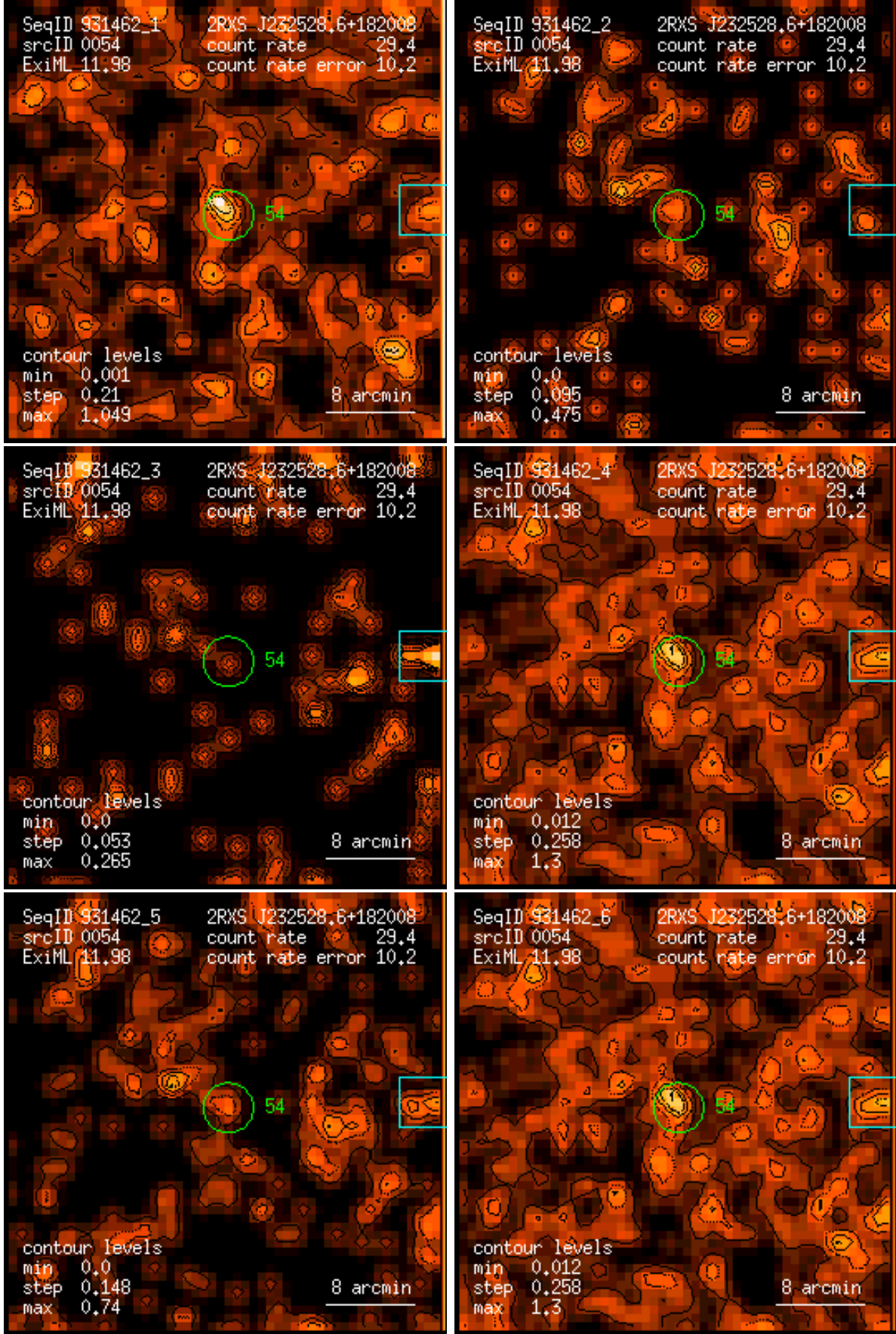
Figure 54: RASS 931462: detection 0054: band rate images, Gaussian filter: (1) PSPC channels 11 – 41, (2) 52 – 90, (3) 91 – 201, (4) 11 – 235, (5) 52 – 201, (6) 11 – 201. Broad band rates in counts/ks. Band rate contour levels in counts/ks/arcmin 2 .
