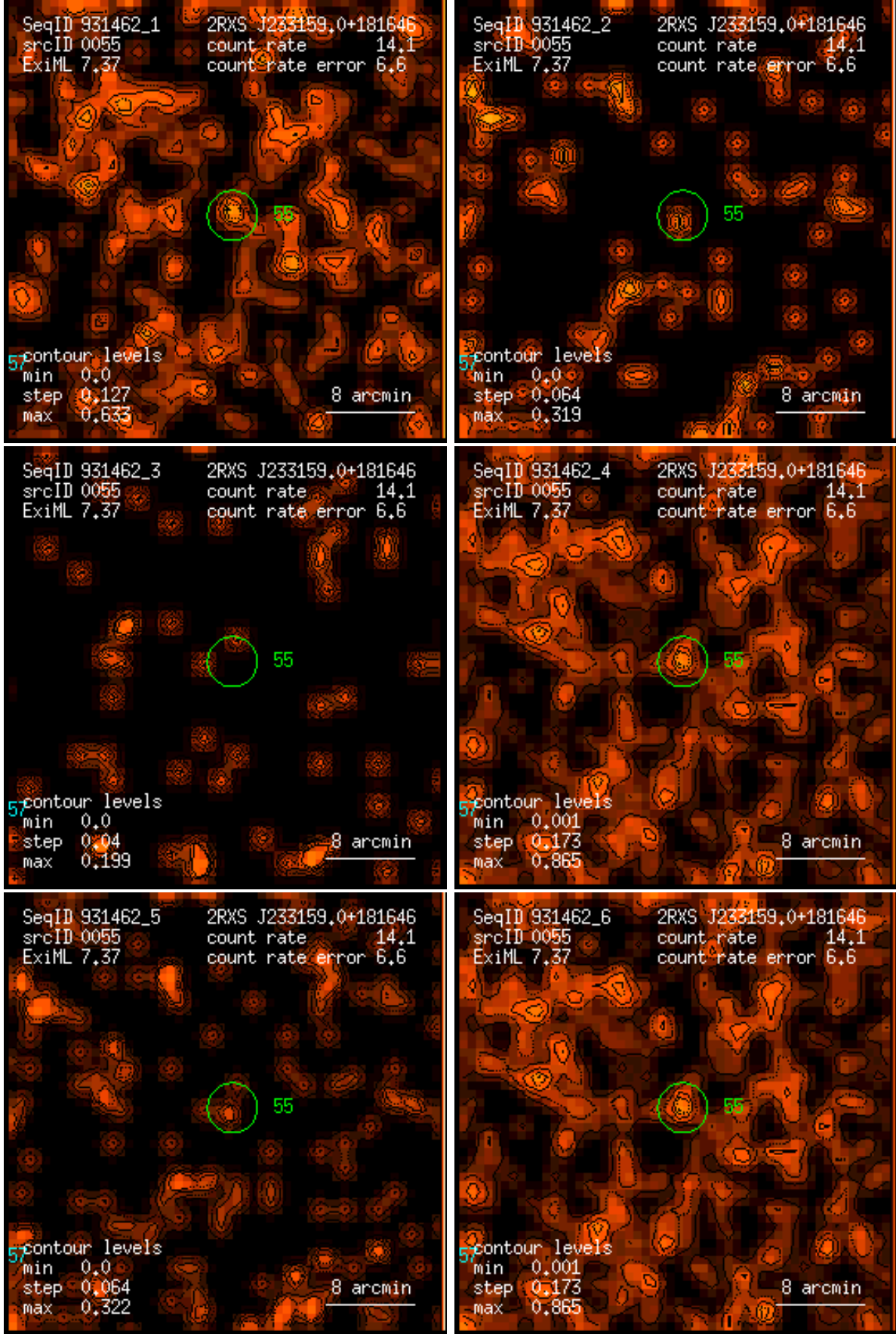
Figure 55: RASS 931462: detection 0055: band rate images, Gaussian filter: (1) PSPC channels 11 – 41, (2) 52 – 90, (3) 91 – 201, (4) 11 – 235, (5) 52 – 201, (6) 11 – 201. Broad band rates in counts/ks. Band rate contour levels in counts/ks/arcmin 2 .
