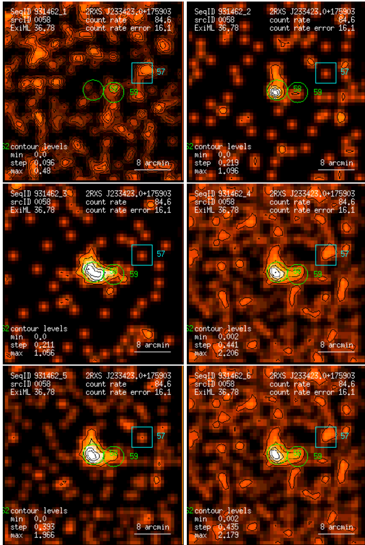
Figure 58: RASS 931462: detection 0058: band rate images, Gaussian filter: (1) PSPC channels 11 – 41, (2) 52 – 90, (3) 91 – 201, (4) 11 – 235, (5) 52 – 201, (6) 11 – 201. Broad band rates in counts/ks. Band rate contour levels in counts/ks/arcmin 2 .
