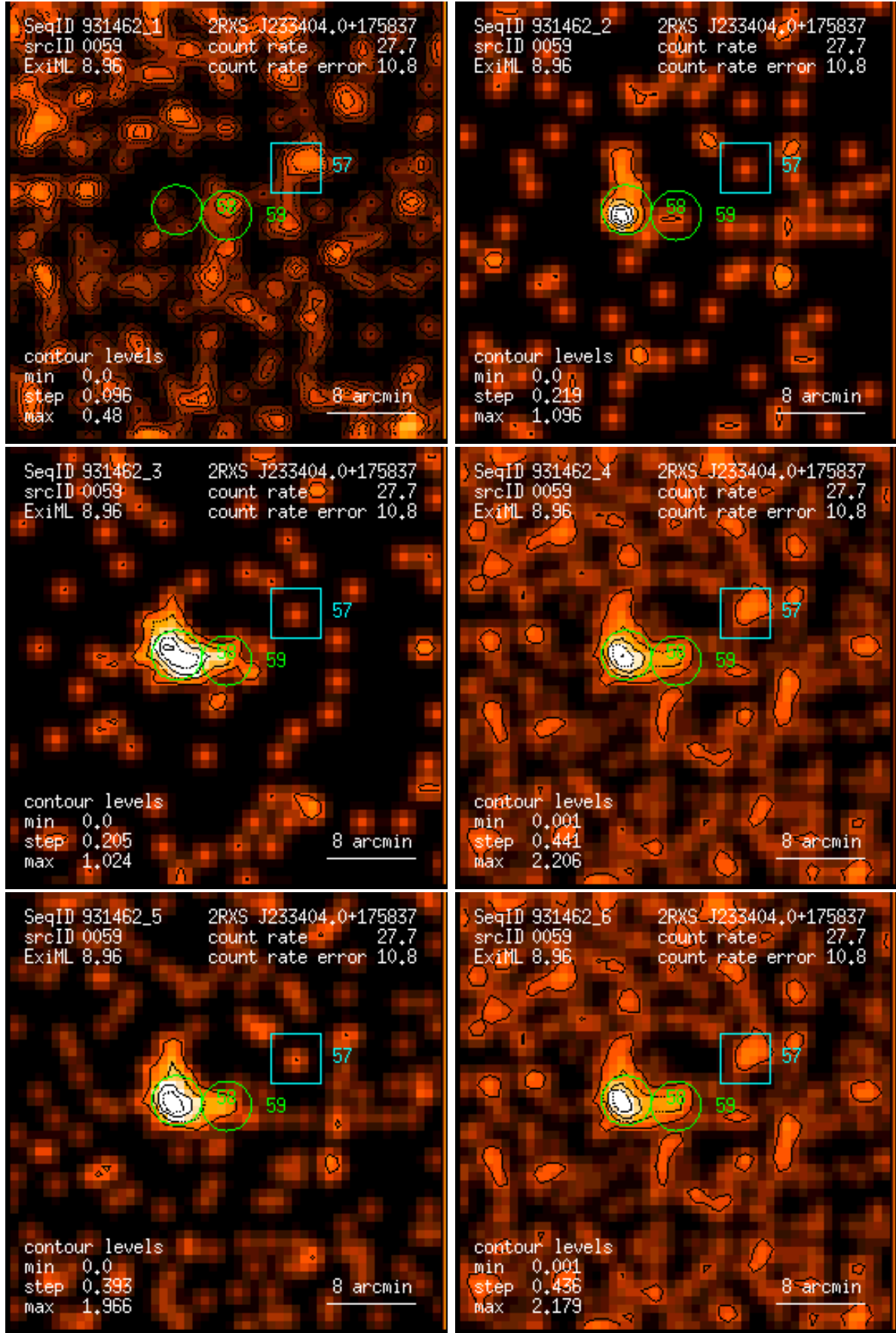
Figure 59: RASS 931462: detection 0059: band rate images, Gaussian filter: (1) PSPC channels 11 – 41, (2) 52 – 90, (3) 91 – 201, (4) 11 – 235, (5) 52 – 201, (6) 11 – 201. Broad band rates in counts/ks. Band rate contour levels in counts/ks/arcmin 2 .
