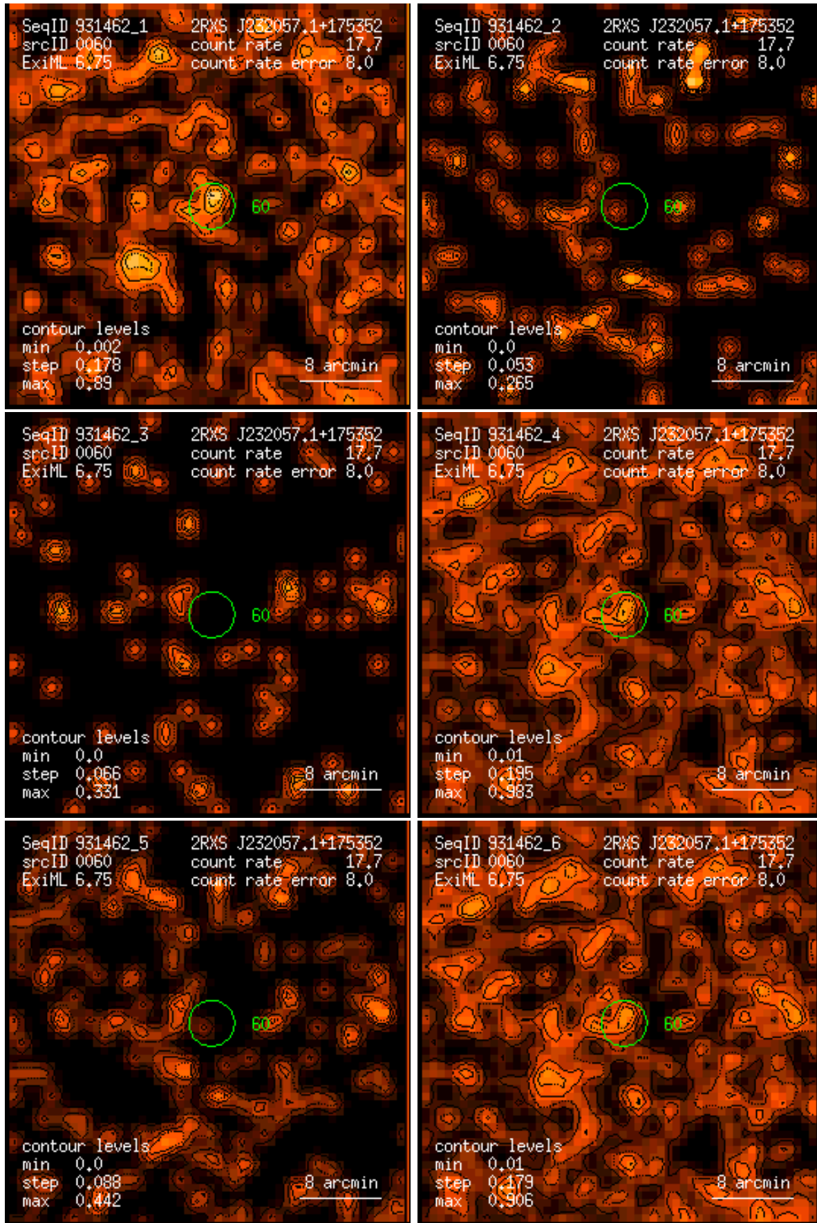
Figure 60: RASS 931462: detection 0060: band rate images, Gaussian filter: (1) PSPC channels 11 – 41, (2) 52 – 90, (3) 91 – 201, (4) 11 – 235, (5) 52 – 201, (6) 11 – 201. Broad band rates in counts/ks. Band rate contour levels in counts/ks/arcmin 2 .
