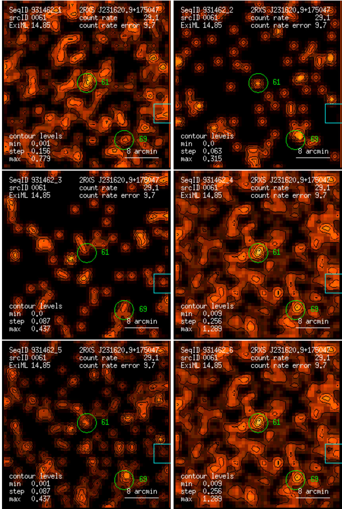
Figure 61: RASS 931462: detection 0061: band rate images, Gaussian filter: (1) PSPC channels 11 – 41, (2) 52 – 90, (3) 91 – 201, (4) 11 – 235, (5) 52 – 201, (6) 11 – 201. Broad band rates in counts/ks. Band rate contour levels in counts/ks/arcmin 2 .
