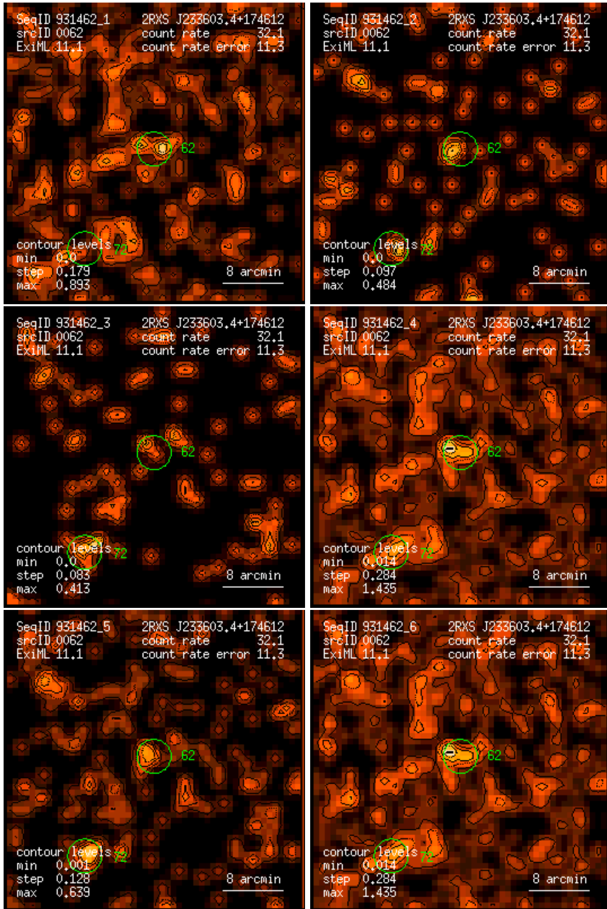
Figure 62: RASS 931462: detection 0062: band rate images, Gaussian filter: (1) PSPC channels 11 – 41, (2) 52 – 90, (3) 91 – 201, (4) 11 – 235, (5) 52 – 201, (6) 11 – 201. Broad band rates in counts/ks. Band rate contour levels in counts/ks/arcmin 2 .
