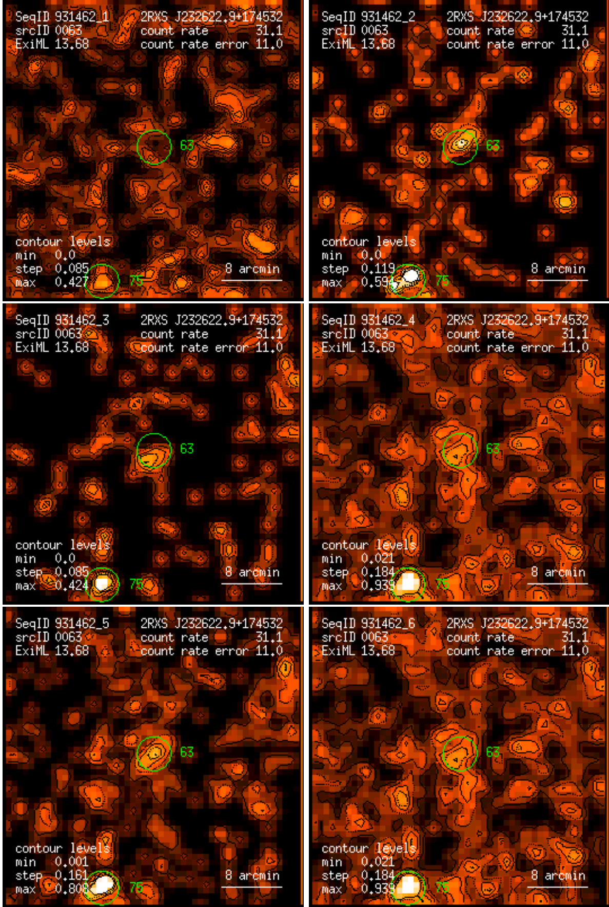
Figure 63: RASS 931462: detection 0063: band rate images, Gaussian filter: (1) PSPC channels 11 – 41, (2) 52 – 90, (3) 91 – 201, (4) 11 – 235, (5) 52 – 201, (6) 11 – 201. Broad band rates in counts/ks. Band rate contour levels in counts/ks/arcmin 2 .
