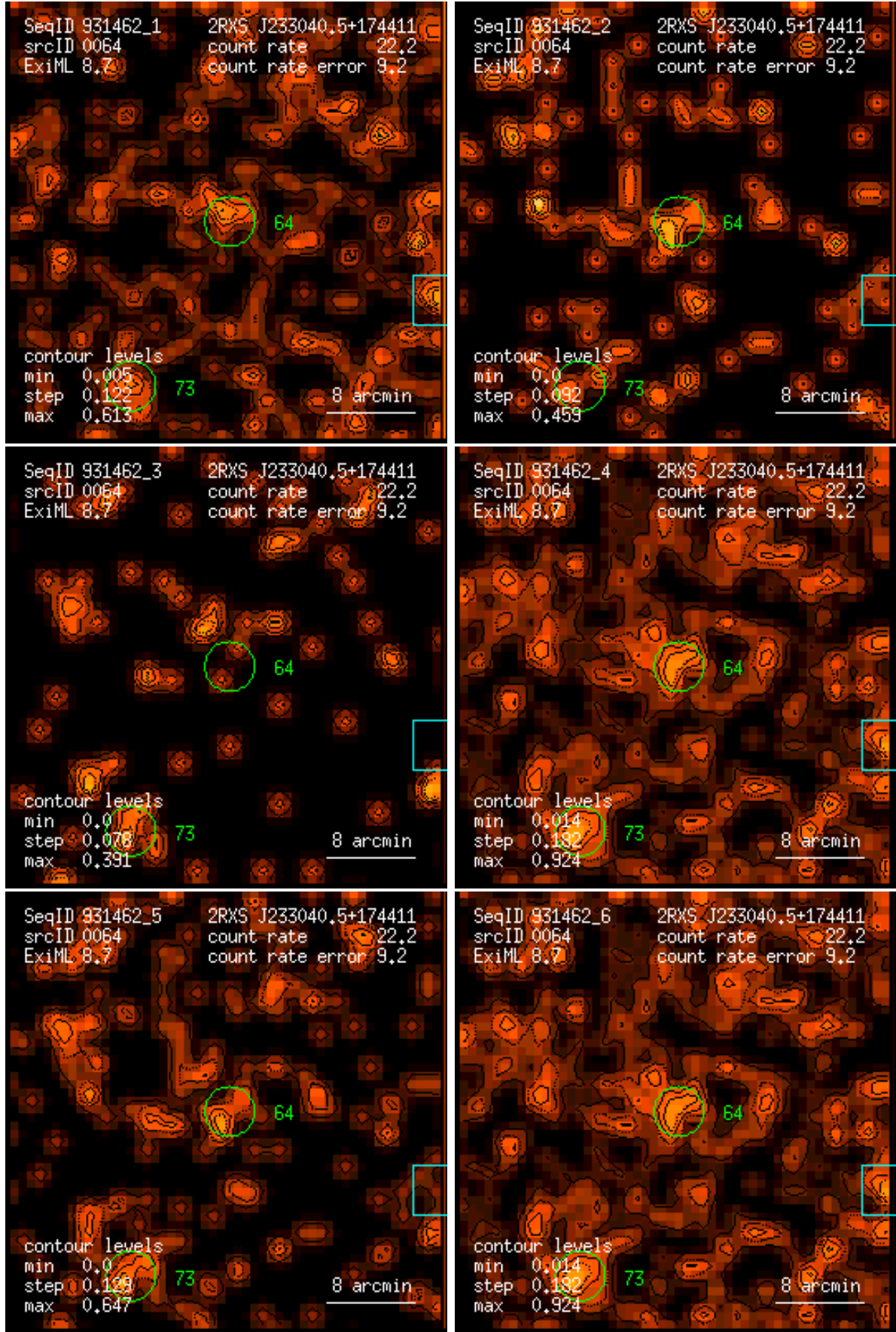
Figure 64: RASS 931462: detection 0064: band rate images, Gaussian filter: (1) PSPC channels 11 – 41, (2) 52 – 90, (3) 91 – 201, (4) 11 – 235, (5) 52 – 201, (6) 11 – 201. Broad band rates in counts/ks. Band rate contour levels in counts/ks/arcmin 2 .
