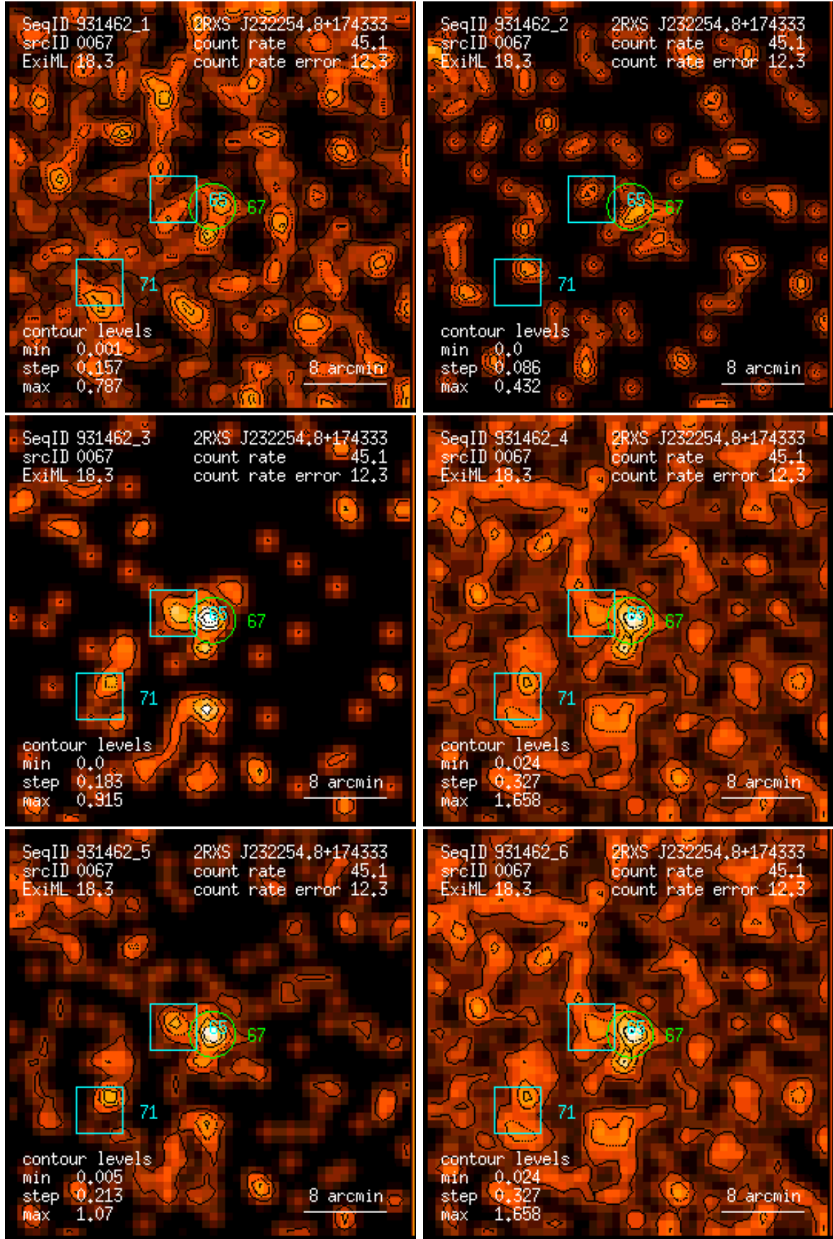
Figure 67: RASS 931462: detection 0067: band rate images, Gaussian filter: (1) PSPC channels 11 – 41, (2) 52 – 90, (3) 91 – 201, (4) 11 – 235, (5) 52 – 201, (6) 11 – 201. Broad band rates in counts/ks. Band rate contour levels in counts/ks/arcmin 2 .
