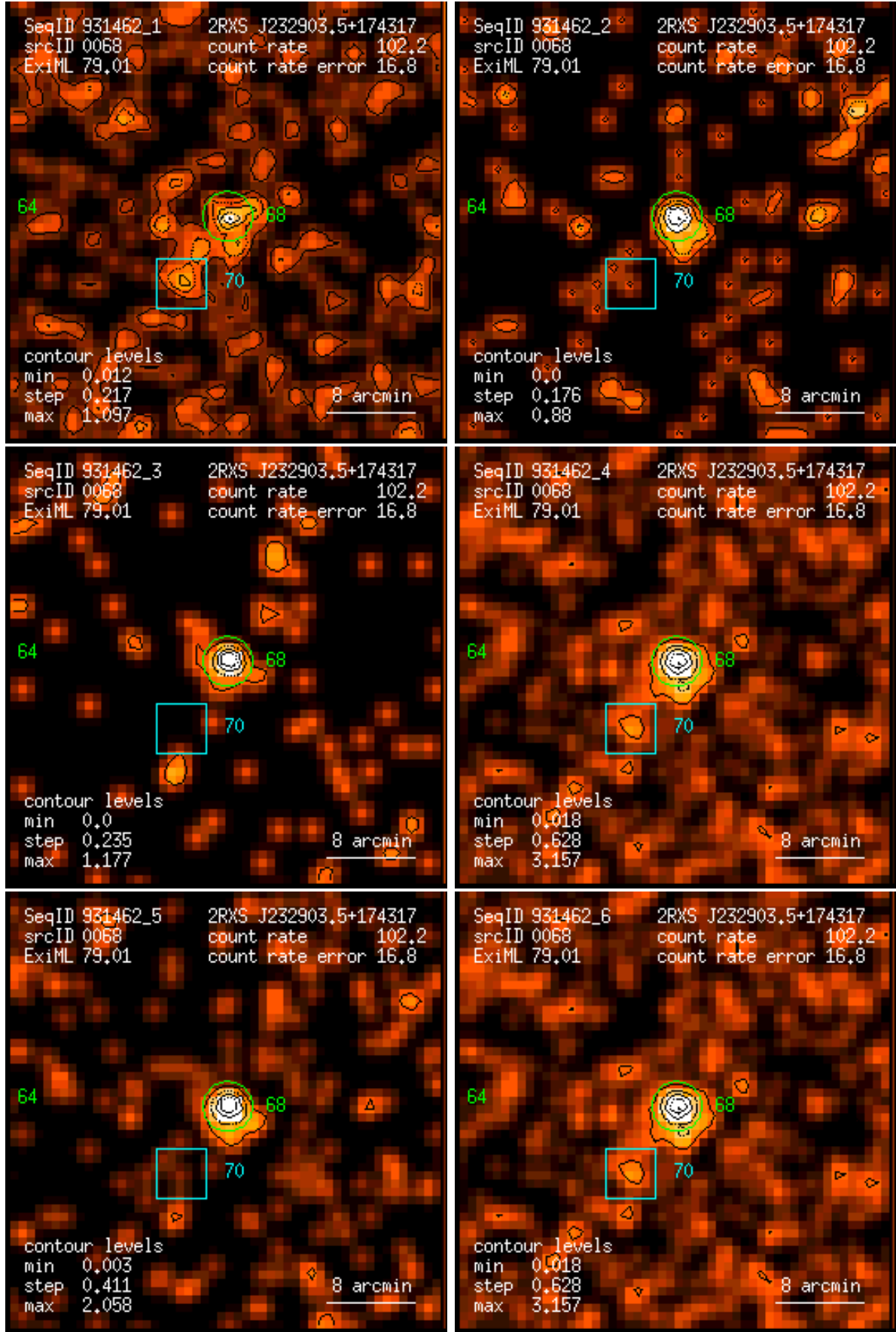
Figure 68: RASS 931462: detection 0068: band rate images, Gaussian filter: (1) PSPC channels 11 – 41, (2) 52 – 90, (3) 91 – 201, (4) 11 – 235, (5) 52 – 201, (6) 11 – 201. Broad band rates in counts/ks. Band rate contour levels in counts/ks/arcmin 2 .
