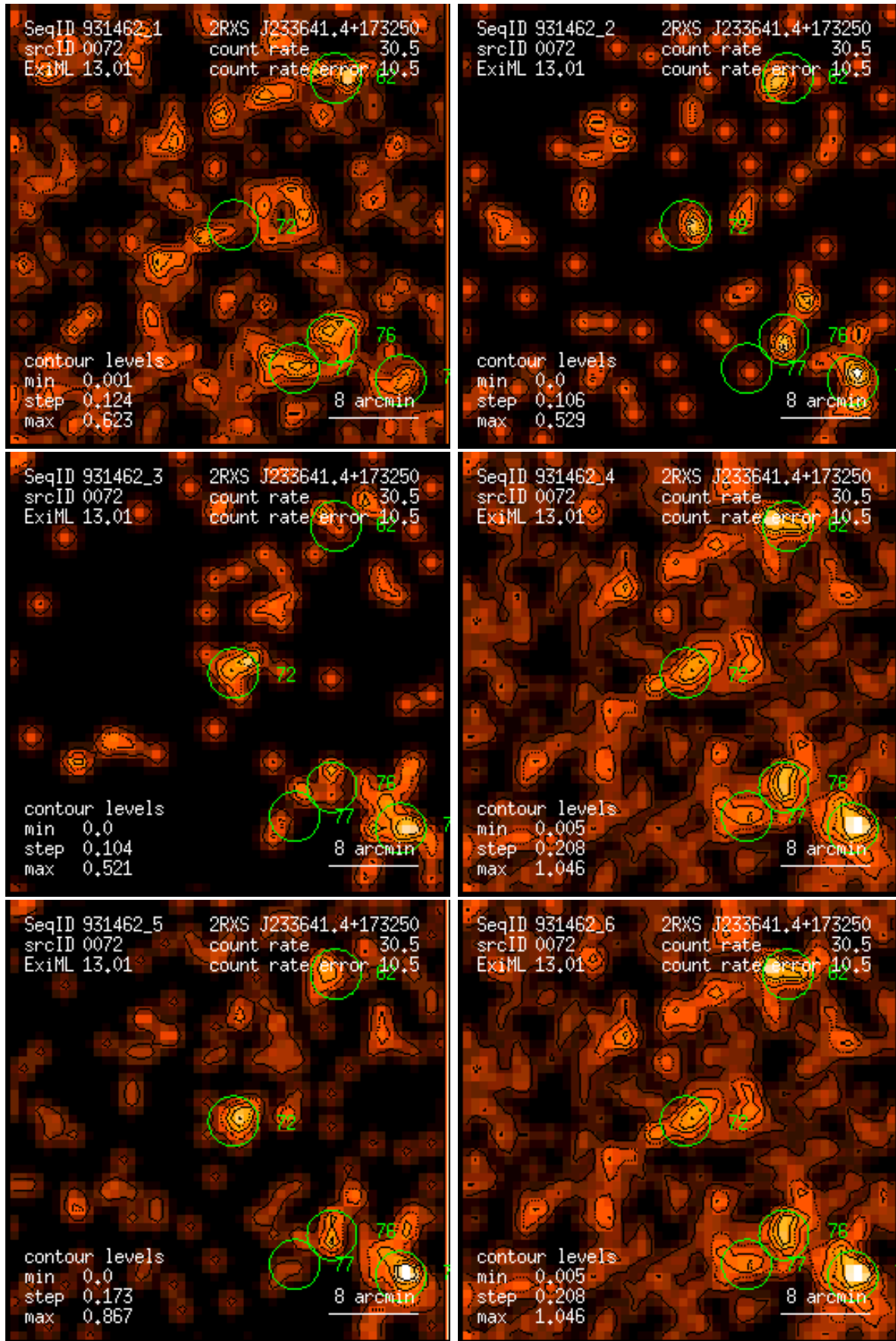
Figure 72: RASS 931462: detection 0072: band rate images, Gaussian filter: (1) PSPC channels 11 – 41, (2) 52 – 90, (3) 91 – 201, (4) 11 – 235, (5) 52 – 201, (6) 11 – 201. Broad band rates in counts/ks. Band rate contour levels in counts/ks/arcmin 2 .
