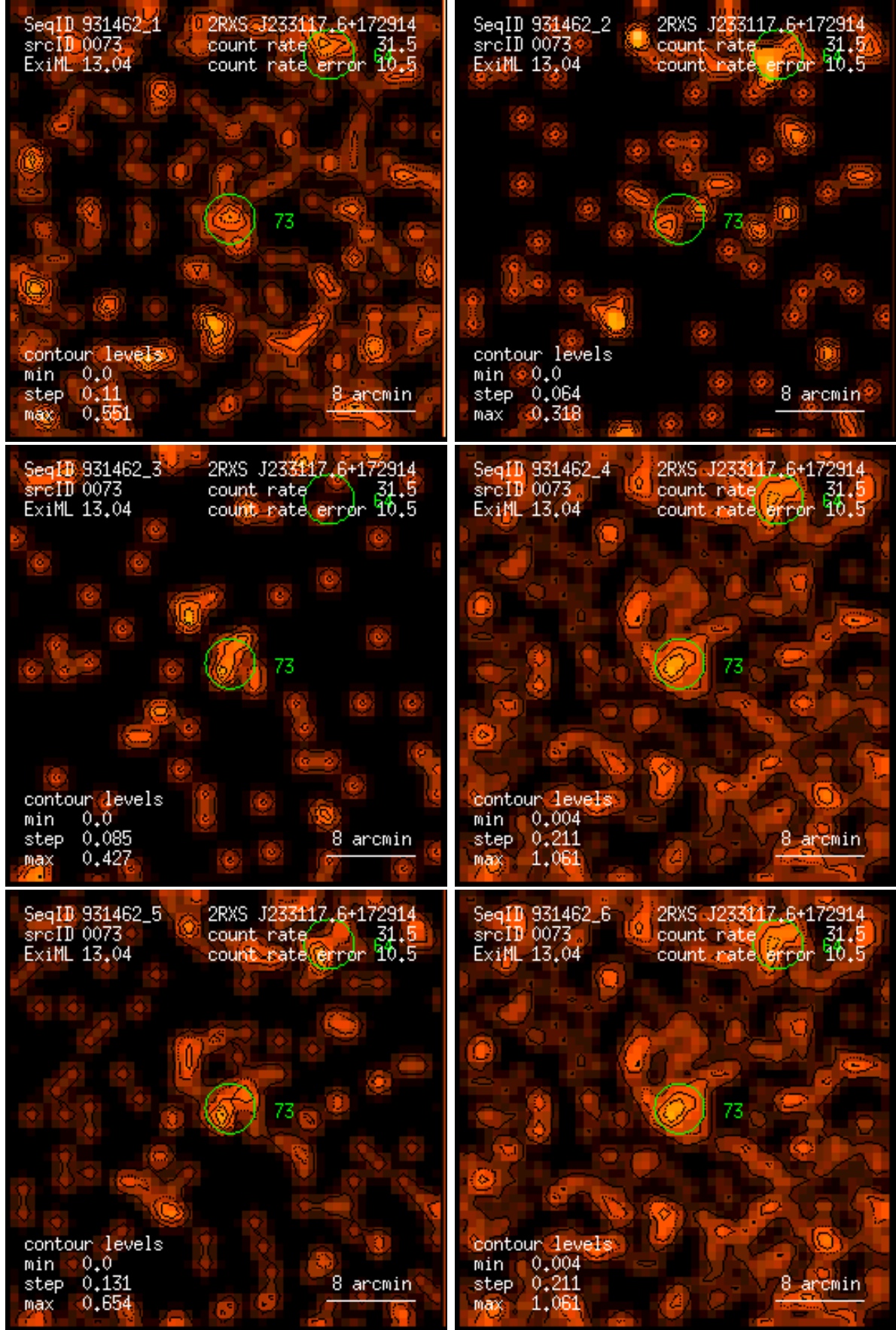
Figure 73: RASS 931462: detection 0073: band rate images, Gaussian filter: (1) PSPC channels 11 – 41, (2) 52 – 90, (3) 91 – 201, (4) 11 – 235, (5) 52 – 201, (6) 11 – 201. Broad band rates in counts/ks. Band rate contour levels in counts/ks/arcmin 2 .
