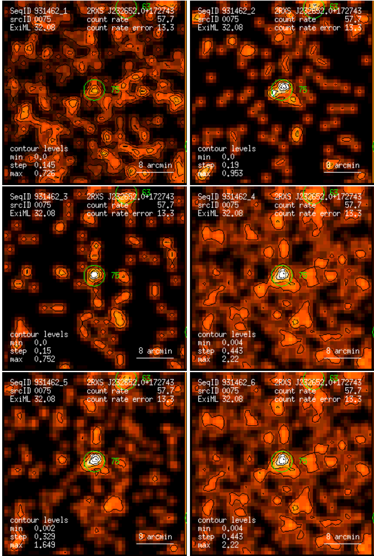
Figure 75: RASS 931462: detection 0075: band rate images, Gaussian filter: (1) PSPC channels 11 – 41, (2) 52 – 90, (3) 91 – 201, (4) 11 – 235, (5) 52 – 201, (6) 11 – 201. Broad band rates in counts/ks. Band rate contour levels in counts/ks/arcmin 2 .
