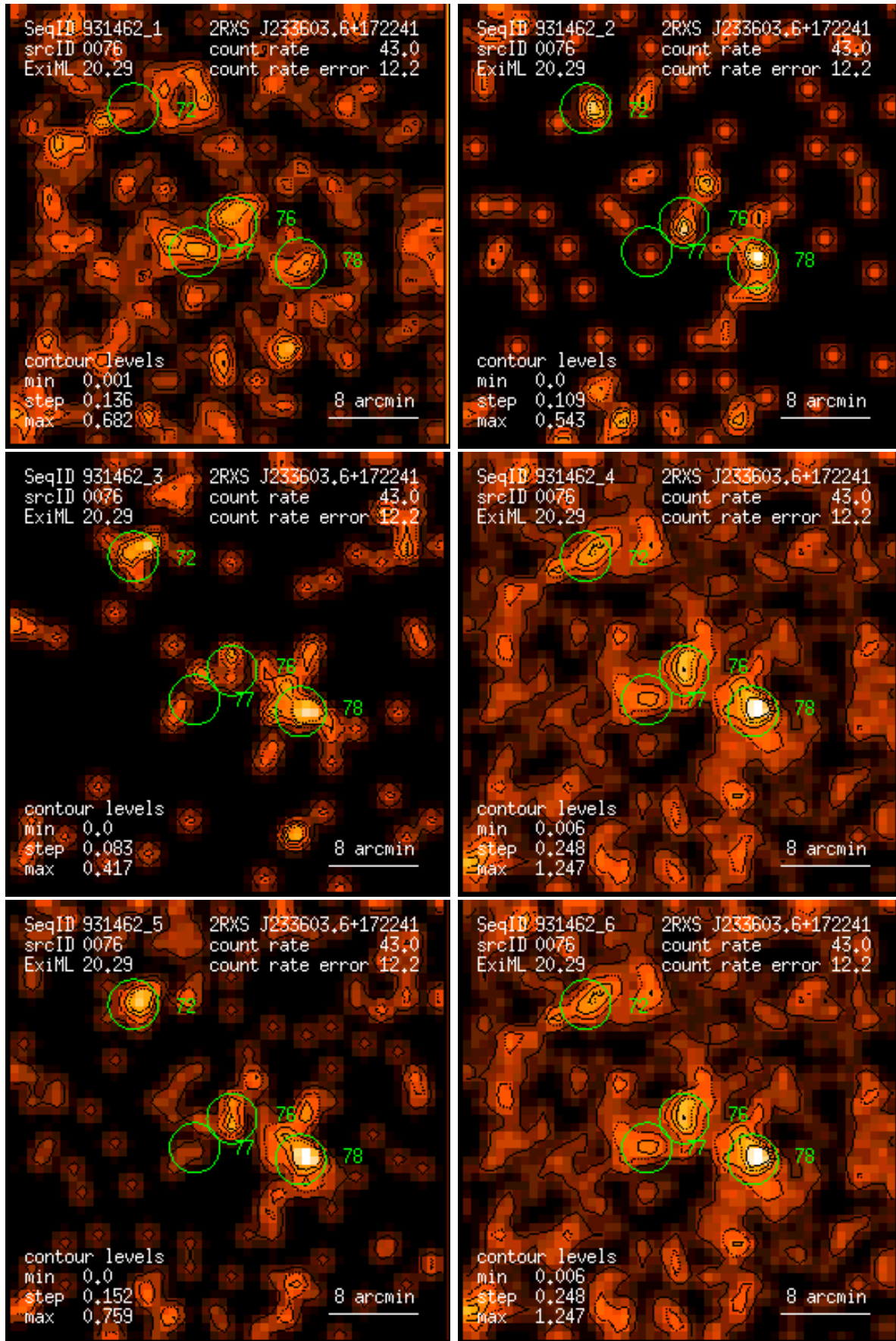
Figure 76: RASS 931462: detection 0076: band rate images, Gaussian filter: (1) PSPC channels 11 – 41, (2) 52 – 90, (3) 91 – 201, (4) 11 – 235, (5) 52 – 201, (6) 11 – 201. Broad band rates in counts/ks. Band rate contour levels in counts/ks/arcmin 2 .
