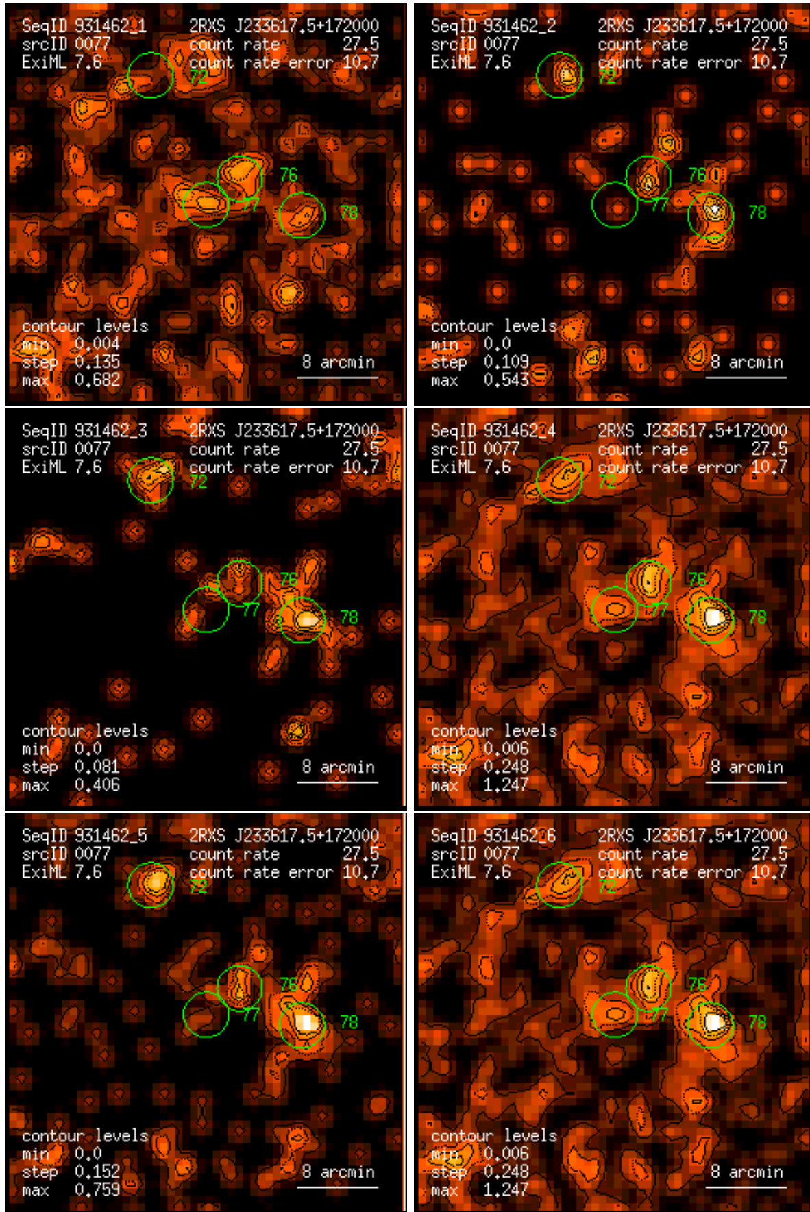
Figure 77: RASS 931462: detection 0077: band rate images, Gaussian filter: (1) PSPC channels 11 – 41, (2) 52 – 90, (3) 91 – 201, (4) 11 – 235, (5) 52 – 201, (6) 11 – 201. Broad band rates in counts/ks. Band rate contour levels in counts/ks/arcmin 2 .
