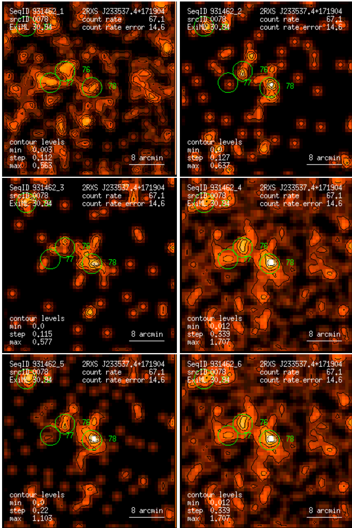
Figure 78: RASS 931462: detection 0078: band rate images, Gaussian filter: (1) PSPC channels 11 – 41, (2) 52 – 90, (3) 91 – 201, (4) 11 – 235, (5) 52 – 201, (6) 11 – 201. Broad band rates in counts/ks. Band rate contour levels in counts/ks/arcmin 2 .
