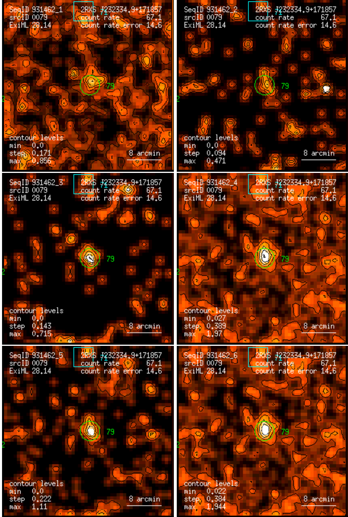
Figure 79: RASS 931462: detection 0079: band rate images, Gaussian filter: (1) PSPC channels 11 – 41, (2) 52 – 90, (3) 91 – 201, (4) 11 – 235, (5) 52 – 201, (6) 11 – 201. Broad band rates in counts/ks. Band rate contour levels in counts/ks/arcmin 2 .
