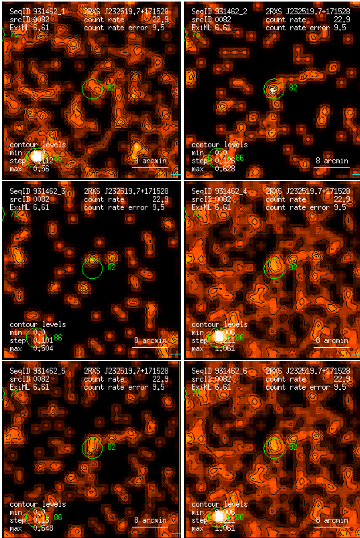
Figure 82: RASS 931462: detection 0082: band rate images, Gaussian filter: (1) PSPC channels 11 – 41, (2) 52 – 90, (3) 91 – 201, (4) 11 – 235, (5) 52 – 201, (6) 11 – 201. Broad band rates in counts/ks. Band rate contour levels in counts/ks/arcmin 2 .
