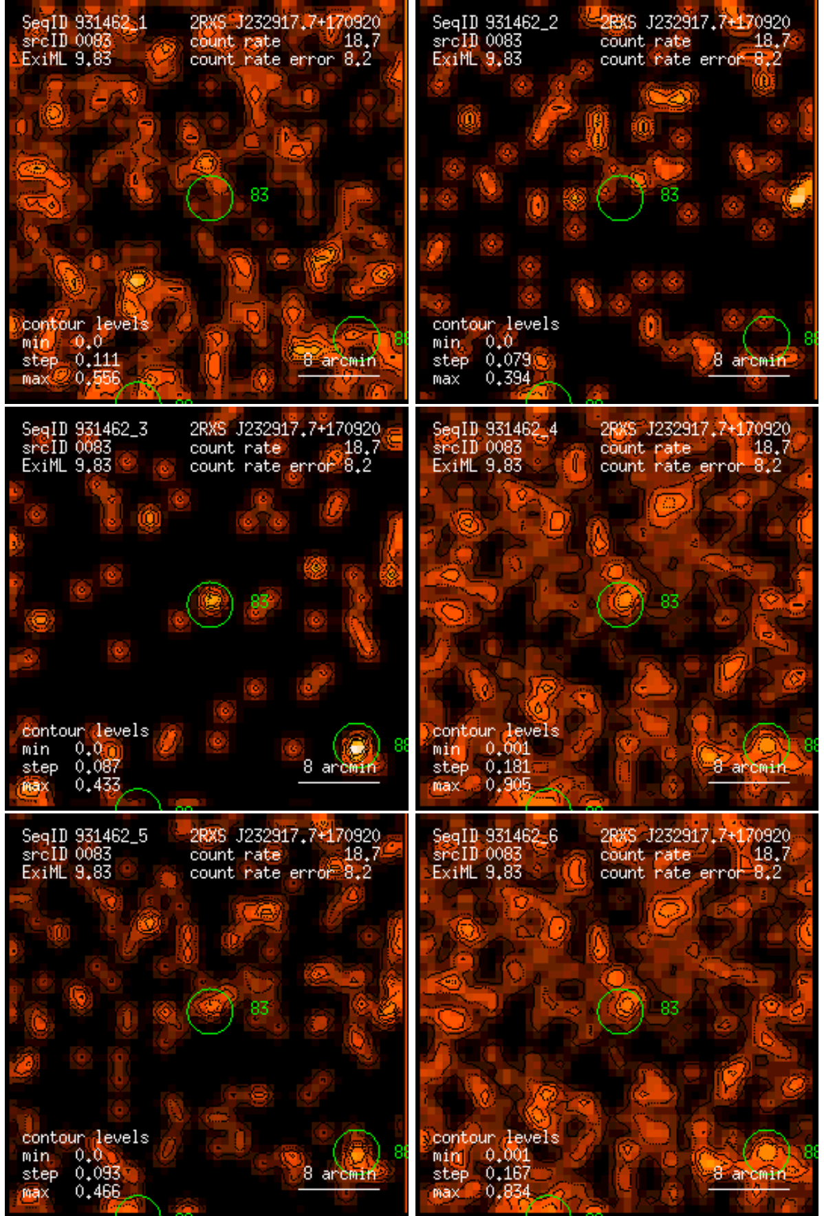
Figure 83: RASS 931462: detection 0083: band rate images, Gaussian filter: (1) PSPC channels 11 – 41, (2) 52 – 90, (3) 91 – 201, (4) 11 – 235, (5) 52 – 201, (6) 11 – 201. Broad band rates in counts/ks. Band rate contour levels in counts/ks/arcmin 2 .
