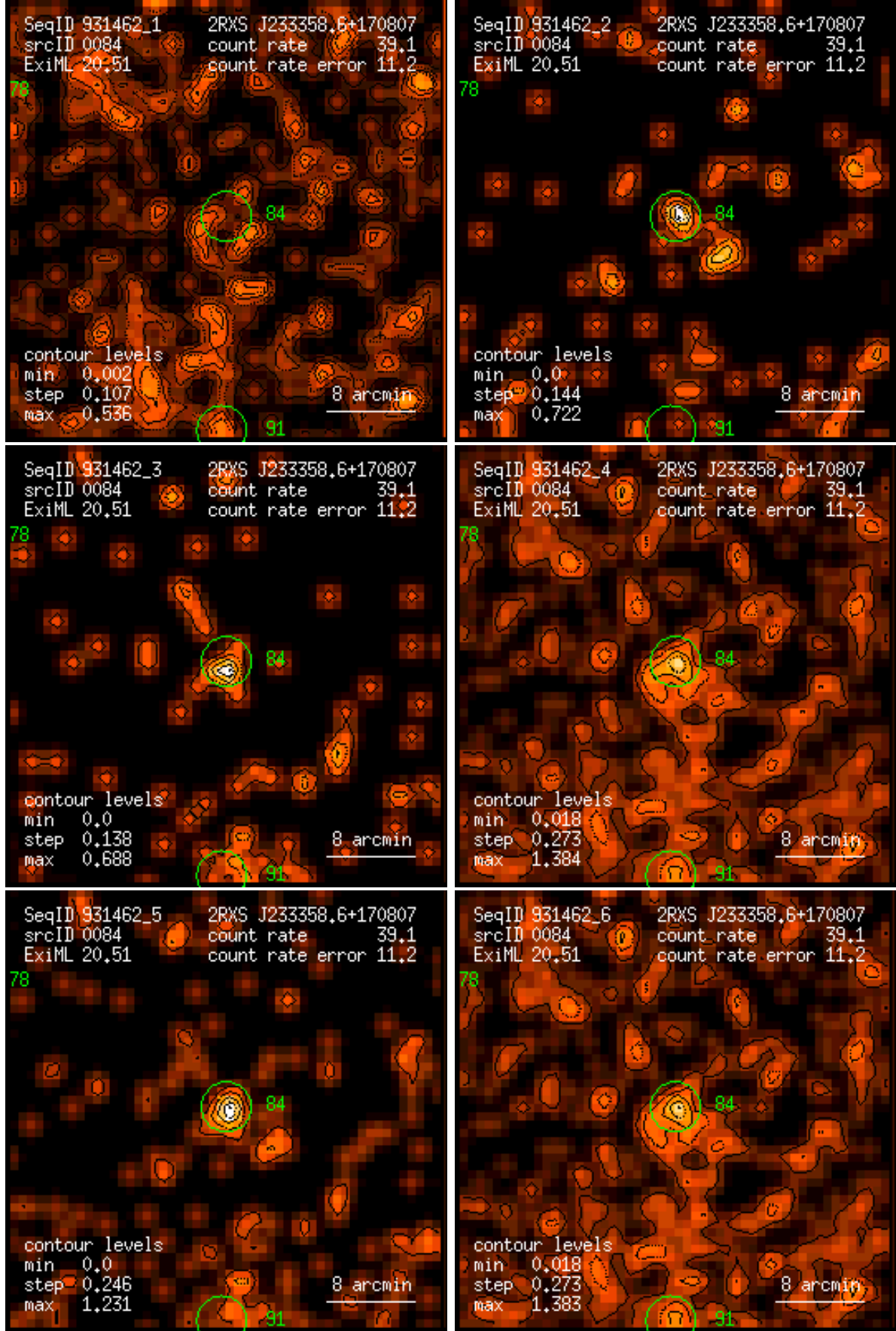
Figure 84: RASS 931462: detection 0084: band rate images, Gaussian filter: (1) PSPC channels 11 – 41, (2) 52 – 90, (3) 91 – 201, (4) 11 – 235, (5) 52 – 201, (6) 11 – 201. Broad band rates in counts/ks. Band rate contour levels in counts/ks/arcmin 2 .
