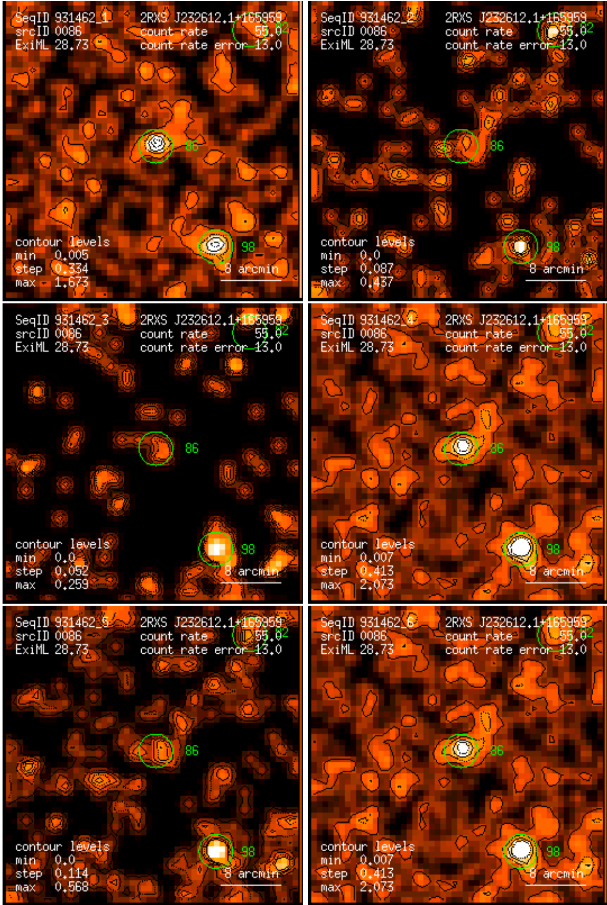
Figure 86: RASS 931462: detection 0086: band rate images, Gaussian filter: (1) PSPC channels 11 – 41, (2) 52 – 90, (3) 91 – 201, (4) 11 – 235, (5) 52 – 201, (6) 11 – 201. Broad band rates in counts/ks. Band rate contour levels in counts/ks/arcmin 2 .
