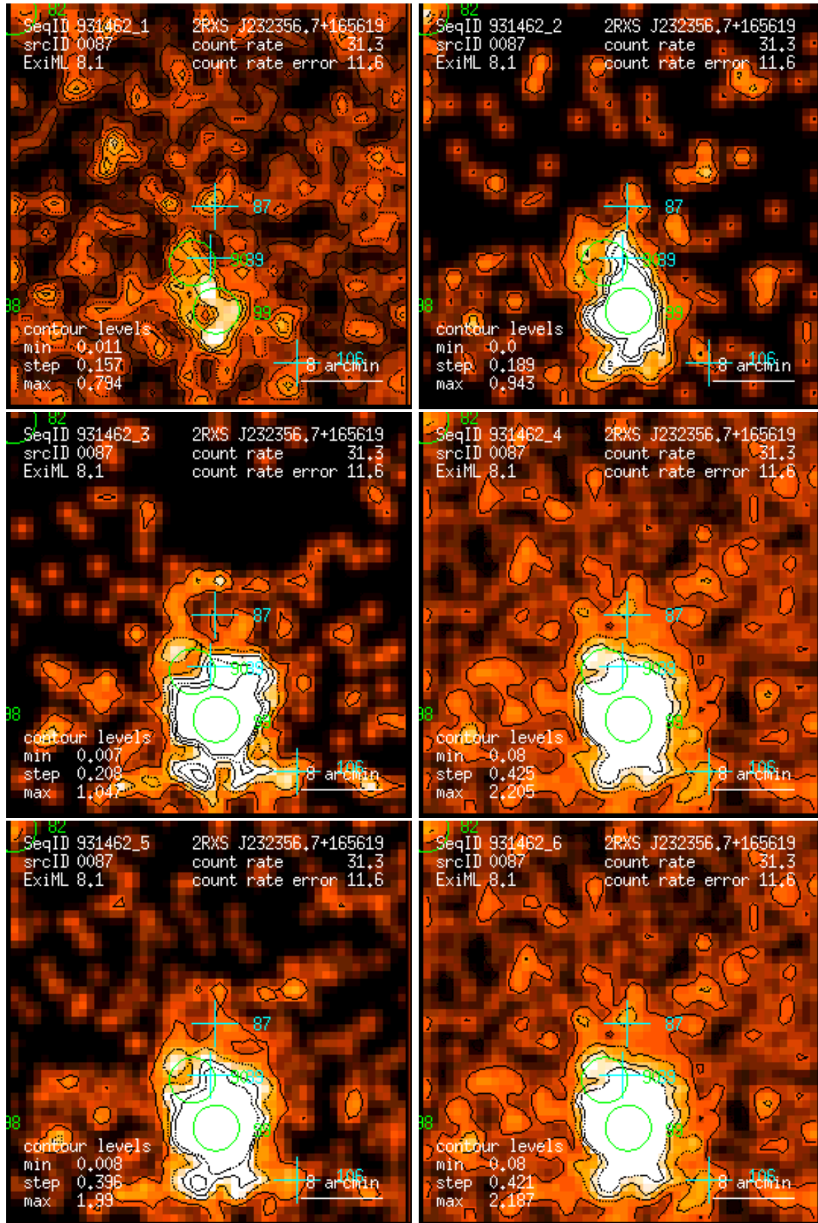
Figure 87: RASS 931462: detection 0087: band rate images, Gaussian filter: (1) PSPC channels 11 – 41, (2) 52 – 90, (3) 91 – 201, (4) 11 – 235, (5) 52 – 201, (6) 11 – 201. Broad band rates in counts/ks. Band rate contour levels in counts/ks/arcmin 2 .
