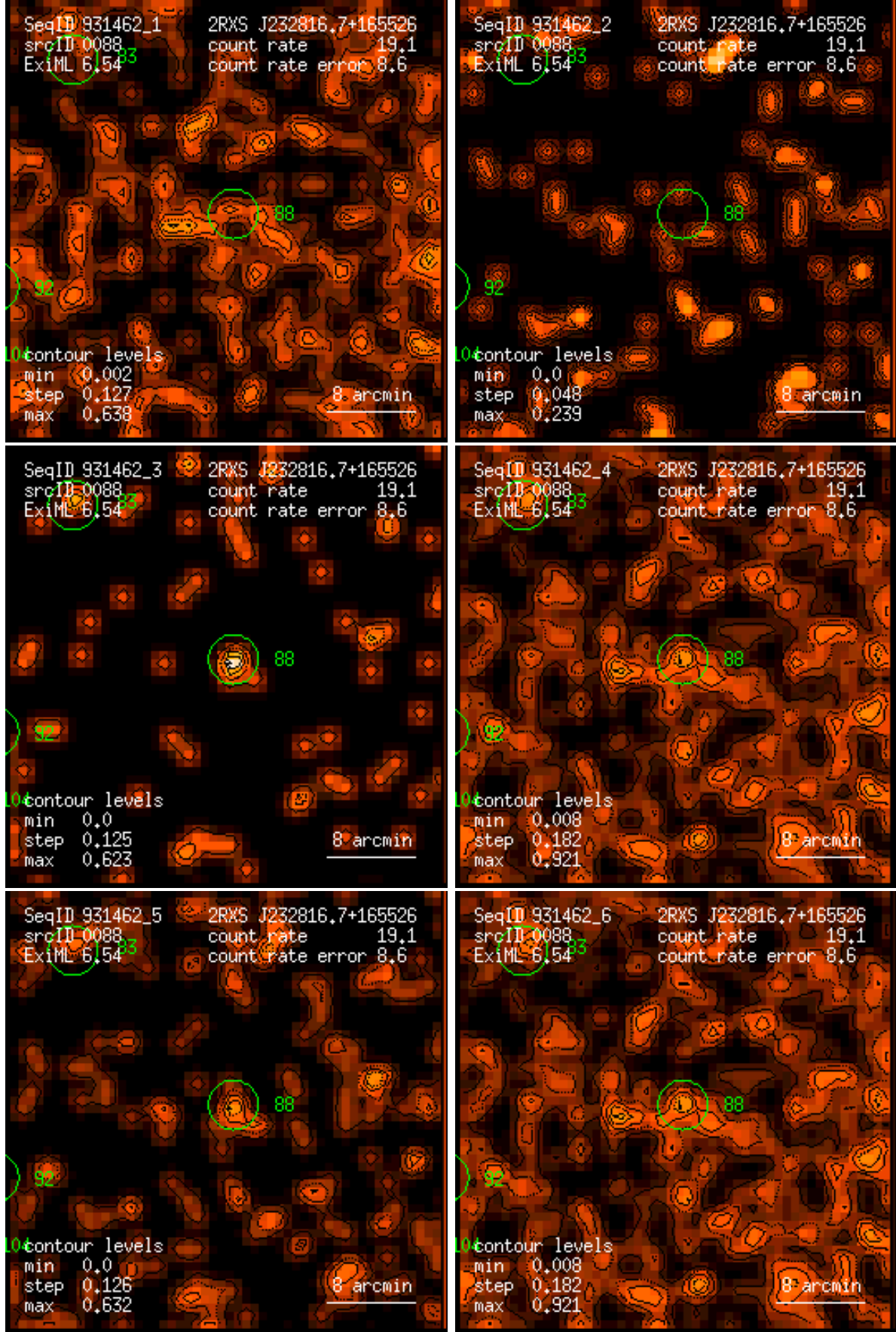
Figure 88: RASS 931462: detection 0088: band rate images, Gaussian filter: (1) PSPC channels 11 – 41, (2) 52 – 90, (3) 91 – 201, (4) 11 – 235, (5) 52 – 201, (6) 11 – 201. Broad band rates in counts/ks. Band rate contour levels in counts/ks/arcmin 2 .
