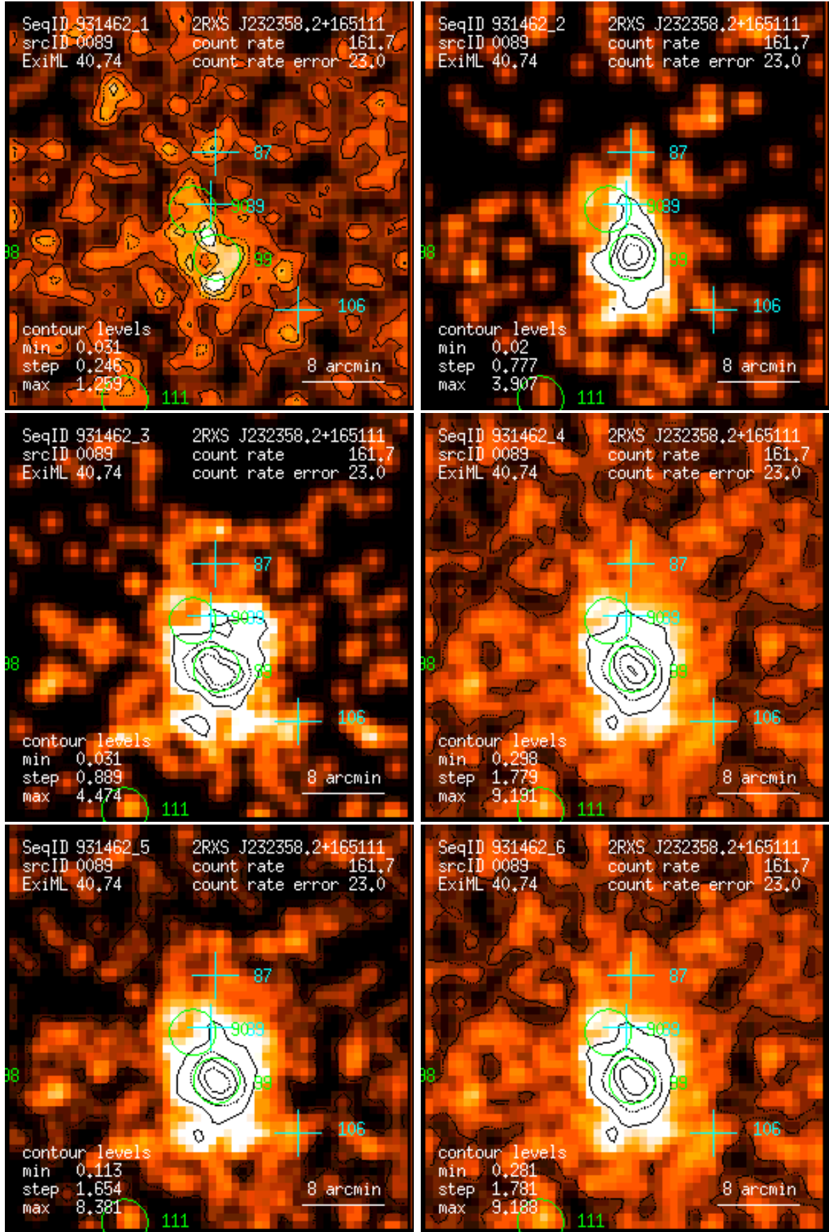
Figure 89: RASS 931462: detection 0089: band rate images, Gaussian filter: (1) PSPC channels 11 – 41, (2) 52 – 90, (3) 91 – 201, (4) 11 – 235, (5) 52 – 201, (6) 11 – 201. Broad band rates in counts/ks. Band rate contour levels in counts/ks/arcmin 2 .
