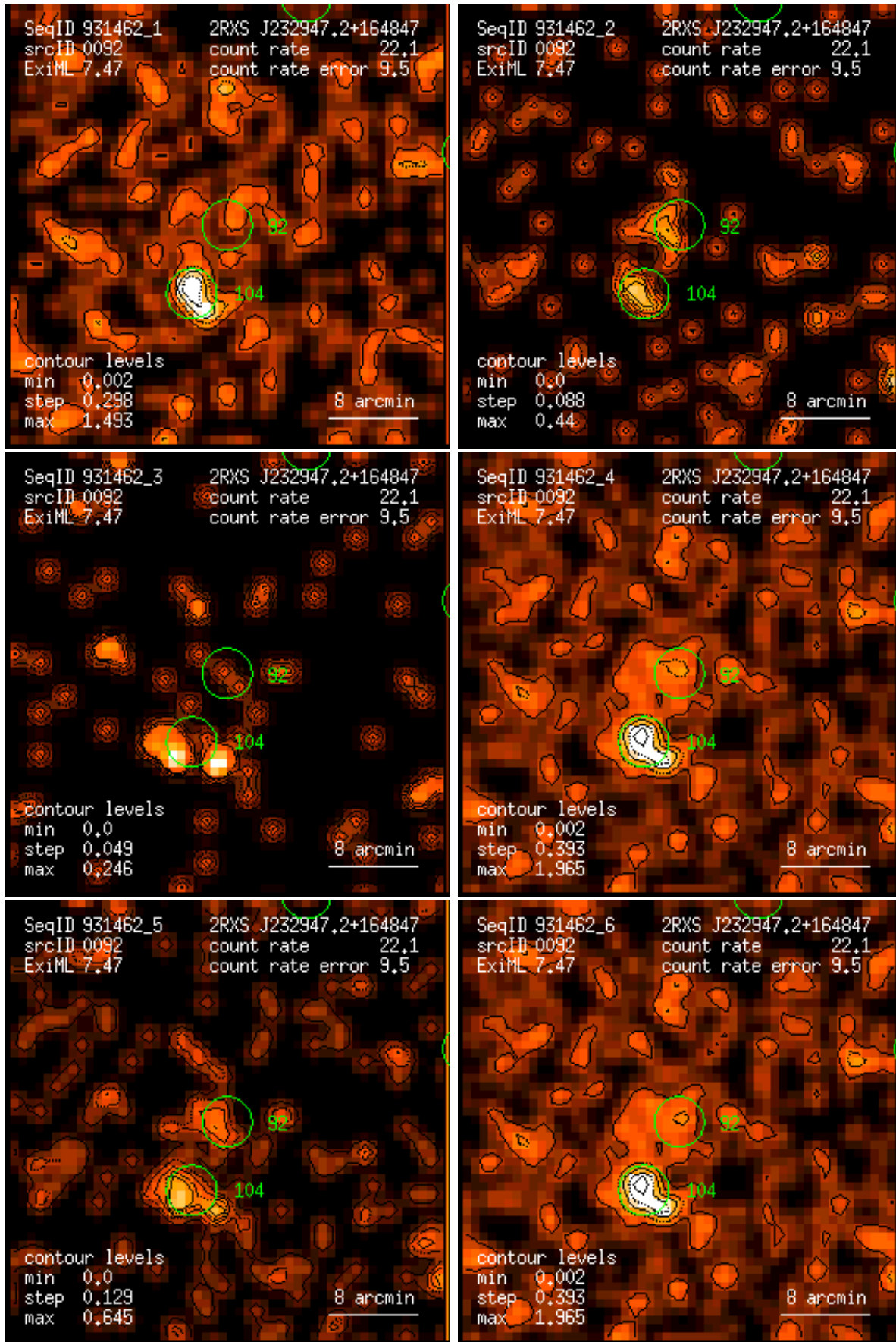
Figure 92: RASS 931462: detection 0092: band rate images, Gaussian filter: (1) PSPC channels 11 – 41, (2) 52 – 90, (3) 91 – 201, (4) 11 – 235, (5) 52 – 201, (6) 11 – 201. Broad band rates in counts/ks. Band rate contour levels in counts/ks/arcmin 2 .
