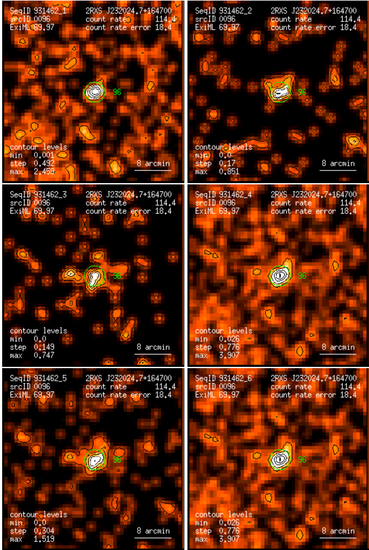
Figure 96: RASS 931462: detection 0096: band rate images, Gaussian filter: (1) PSPC channels 11 – 41, (2) 52 – 90, (3) 91 – 201, (4) 11 – 235, (5) 52 – 201, (6) 11 – 201. Broad band rates in counts/ks. Band rate contour levels in counts/ks/arcmin 2 .
