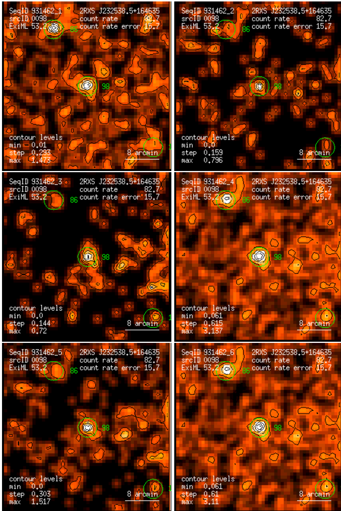
Figure 98: RASS 931462: detection 0098: band rate images, Gaussian filter: (1) PSPC channels 11 – 41, (2) 52 – 90, (3) 91 – 201, (4) 11 – 235, (5) 52 – 201, (6) 11 – 201. Broad band rates in counts/ks. Band rate contour levels in counts/ks/arcmin 2 .
