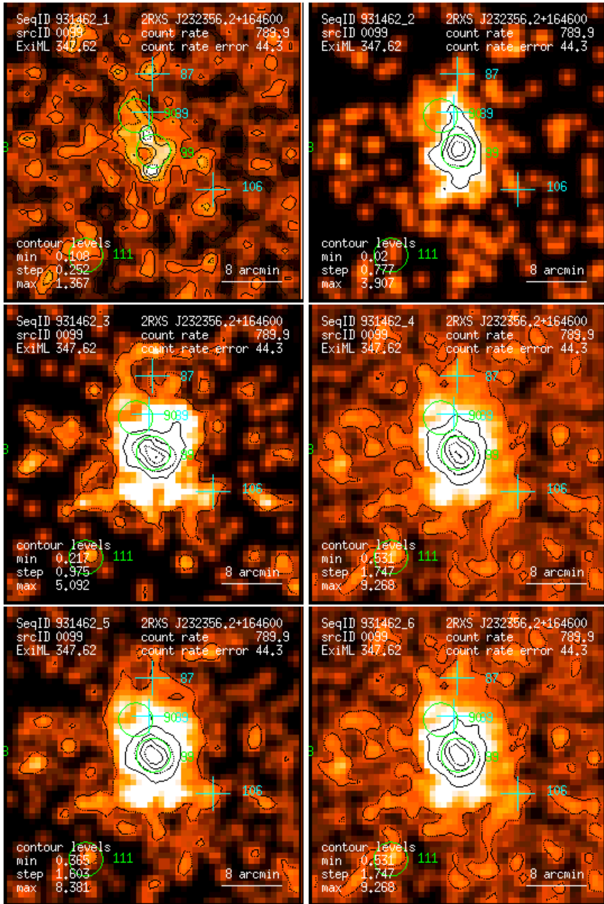
Figure 99: RASS 931462: detection 0099: band rate images, Gaussian filter: (1) PSPC channels 11 – 41, (2) 52 – 90, (3) 91 – 201, (4) 11 – 235, (5) 52 – 201, (6) 11 – 201. Broad band rates in counts/ks. Band rate contour levels in counts/ks/arcmin 2 .
