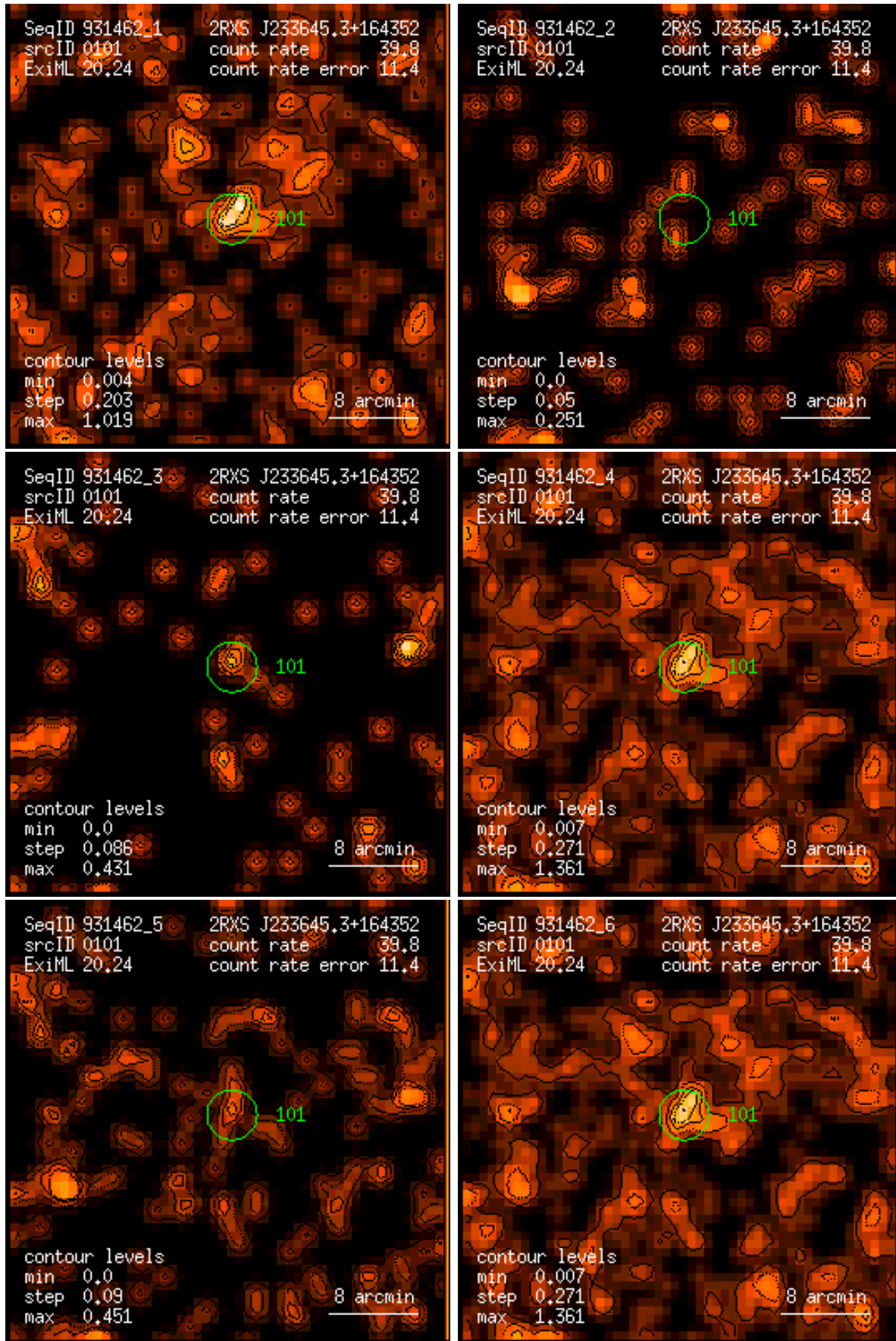
Figure 101: RASS 931462: detection 0101: band rate images, Gaussian filter: (1) PSPC channels 11 – 41, (2) 52 – 90, (3) 91 – 201, (4) 11 – 235, (5) 52 – 201, (6) 11 – 201. Broad band rates in counts/ks. Band rate contour levels in counts/ks/arcmin 2 .
