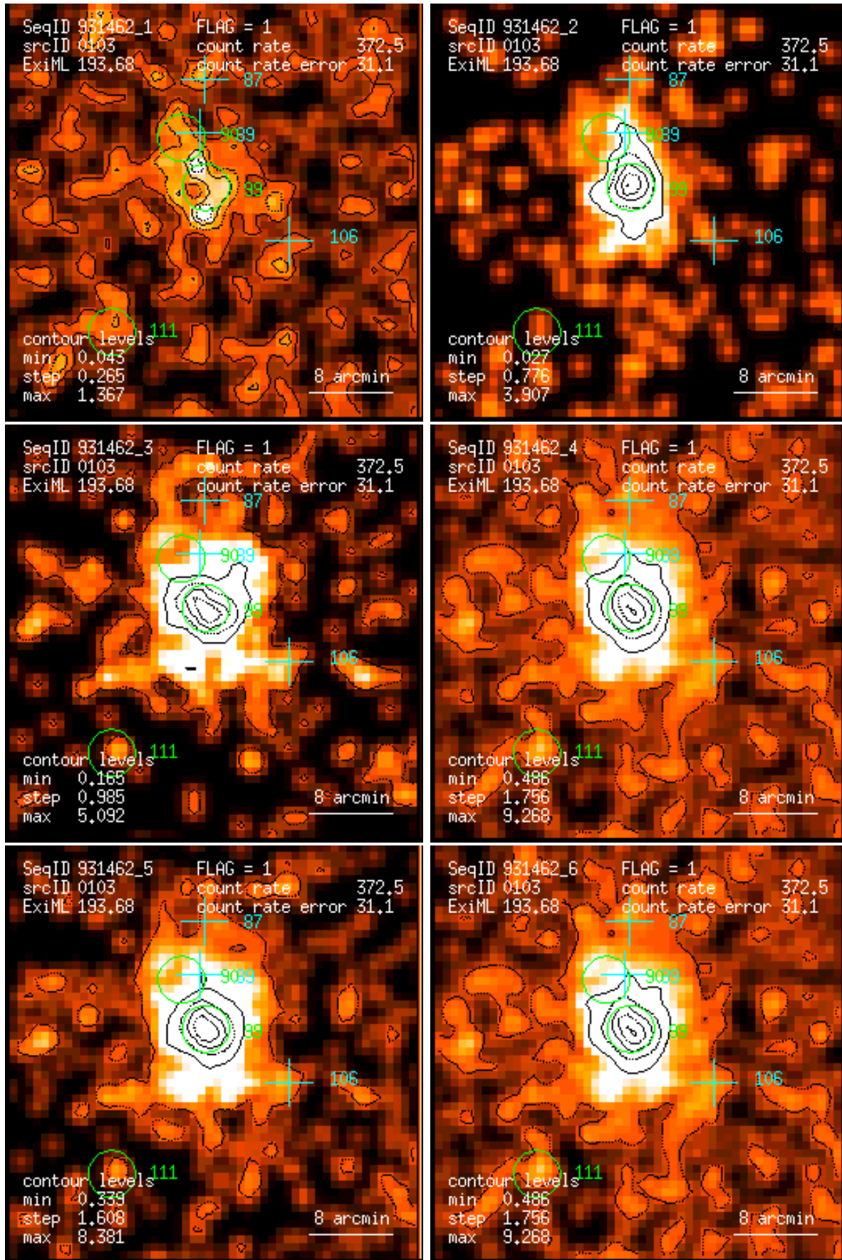
Figure 103: RASS 931462: detection 0103: band rate images, Gaussian filter: (1) PSPC channels 11 – 41, (2) 52 – 90, (3) 91 – 201, (4) 11 – 235, (5) 52 – 201, (6) 11 – 201. Broad band rates in counts/ks. Band rate contour levels in counts/ks/arcmin 2 .
