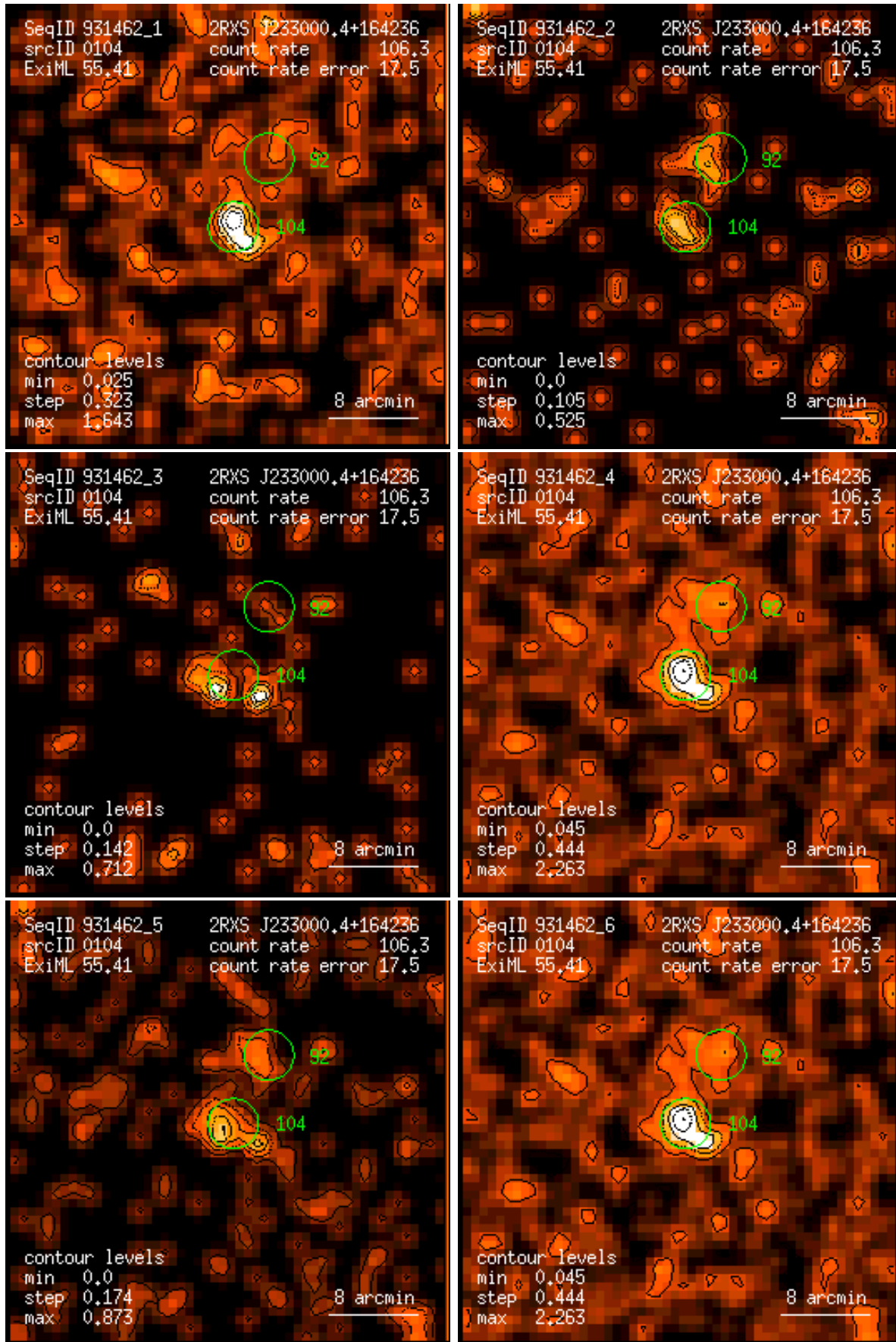
Figure 104: RASS 931462: detection 0104: band rate images, Gaussian filter: (1) PSPC channels 11 – 41, (2) 52 – 90, (3) 91 – 201, (4) 11 – 235, (5) 52 – 201, (6) 11 – 201. Broad band rates in counts/ks. Band rate contour levels in counts/ks/arcmin 2 .
