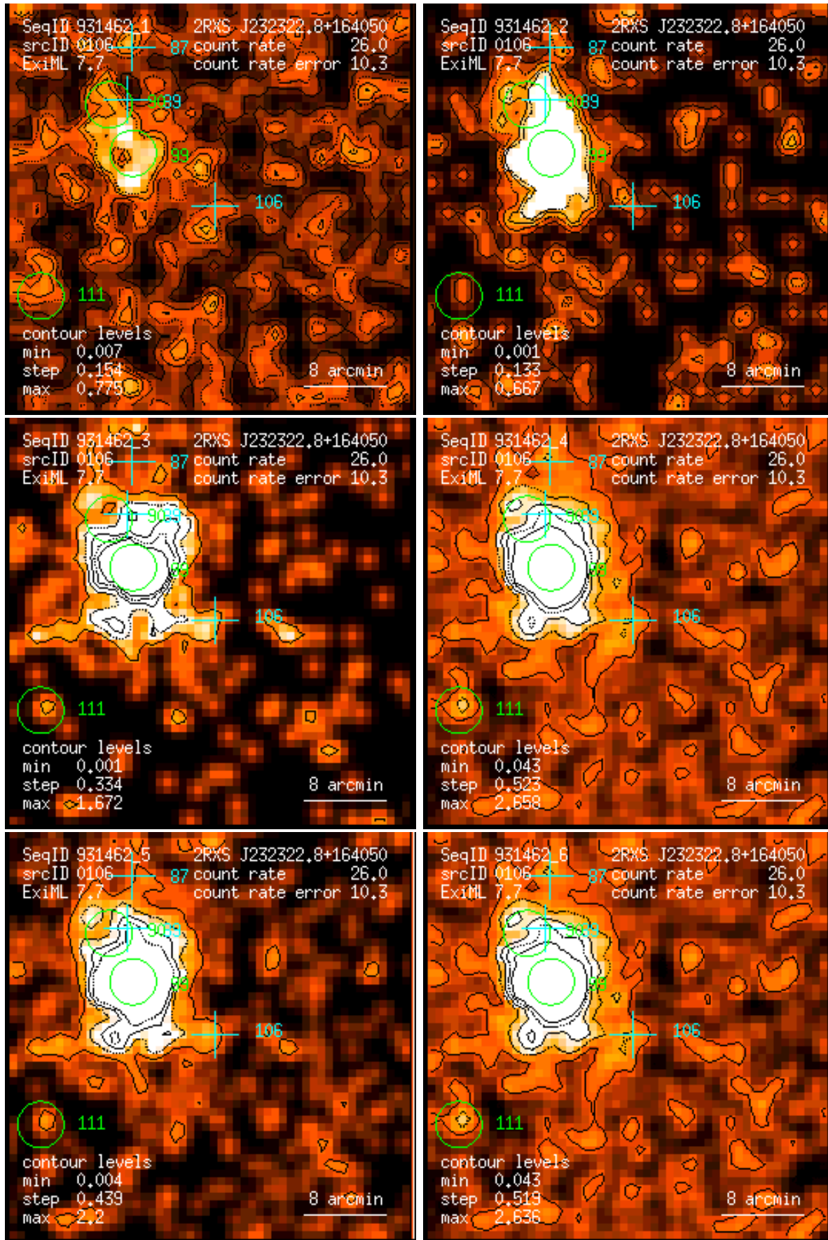
Figure 106: RASS 931462: detection 0106: band rate images, Gaussian filter: (1) PSPC channels 11 – 41, (2) 52 – 90, (3) 91 – 201, (4) 11 – 235, (5) 52 – 201, (6) 11 – 201. Broad band rates in counts/ks. Band rate contour levels in counts/ks/arcmin 2 .
