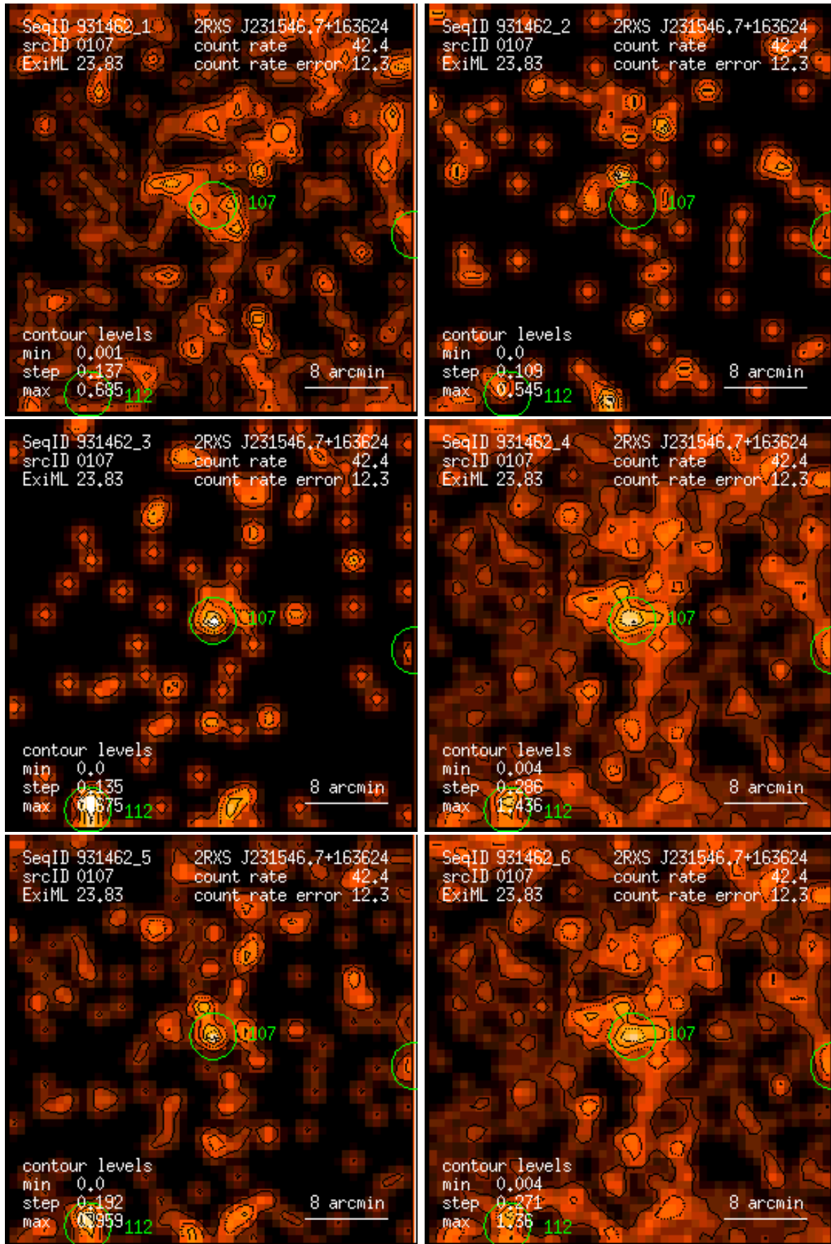
Figure 107: RASS 931462: detection 0107: band rate images, Gaussian filter: (1) PSPC channels 11 – 41, (2) 52 – 90, (3) 91 – 201, (4) 11 – 235, (5) 52 – 201, (6) 11 – 201. Broad band rates in counts/ks. Band rate contour levels in counts/ks/arcmin 2 .
