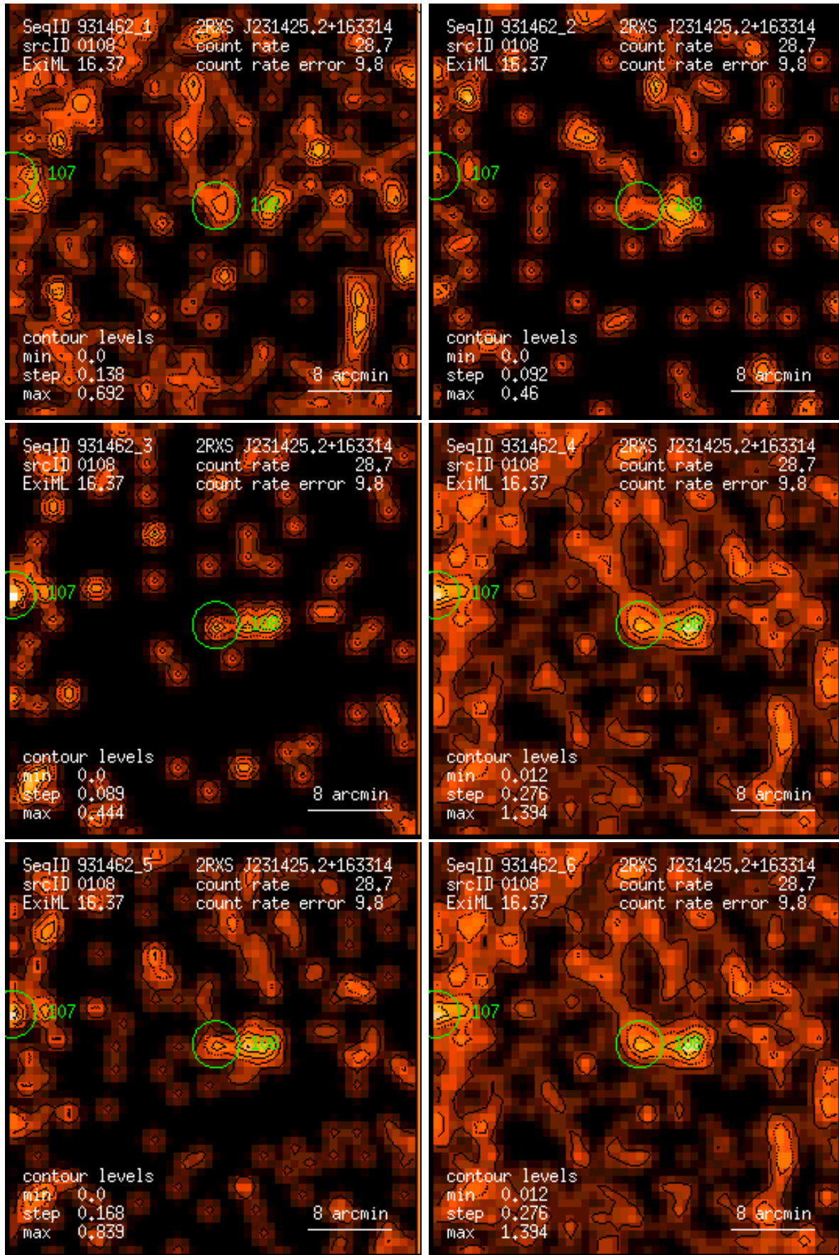
Figure 108: RASS 931462: detection 0108: band rate images, Gaussian filter: (1) PSPC channels 11 – 41, (2) 52 – 90, (3) 91 – 201, (4) 11 – 235, (5) 52 – 201, (6) 11 – 201. Broad band rates in counts/ks. Band rate contour levels in counts/ks/arcmin 2 .
