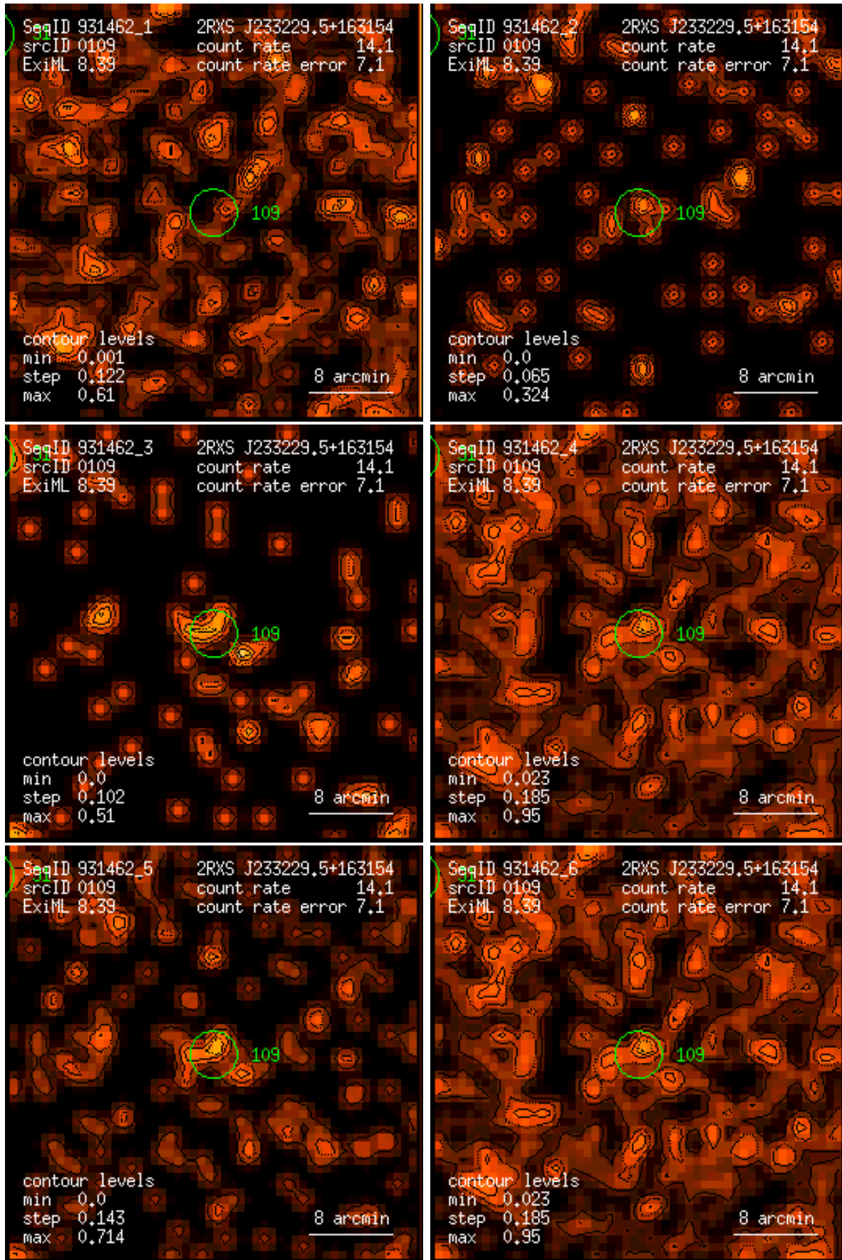
Figure 109: RASS 931462: detection 0109: band rate images, Gaussian filter: (1) PSPC channels 11 – 41, (2) 52 – 90, (3) 91 – 201, (4) 11 – 235, (5) 52 – 201, (6) 11 – 201. Broad band rates in counts/ks. Band rate contour levels in counts/ks/arcmin 2 .
