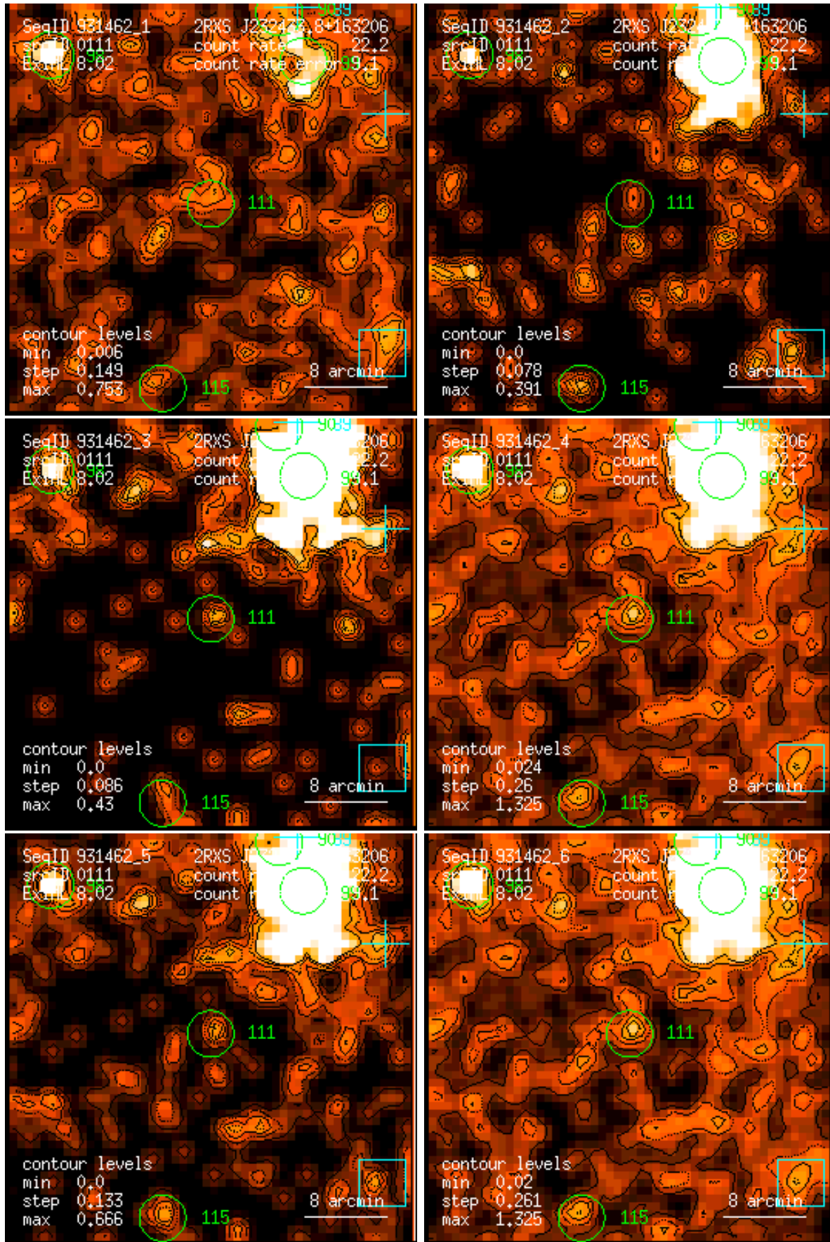
Figure 111: RASS 931462: detection 0111: band rate images, Gaussian filter: (1) PSPC channels 11 – 41, (2) 52 – 90, (3) 91 – 201, (4) 11 – 235, (5) 52 – 201, (6) 11 – 201. Broad band rates in counts/ks. Band rate contour levels in counts/ks/arcmin 2 .
