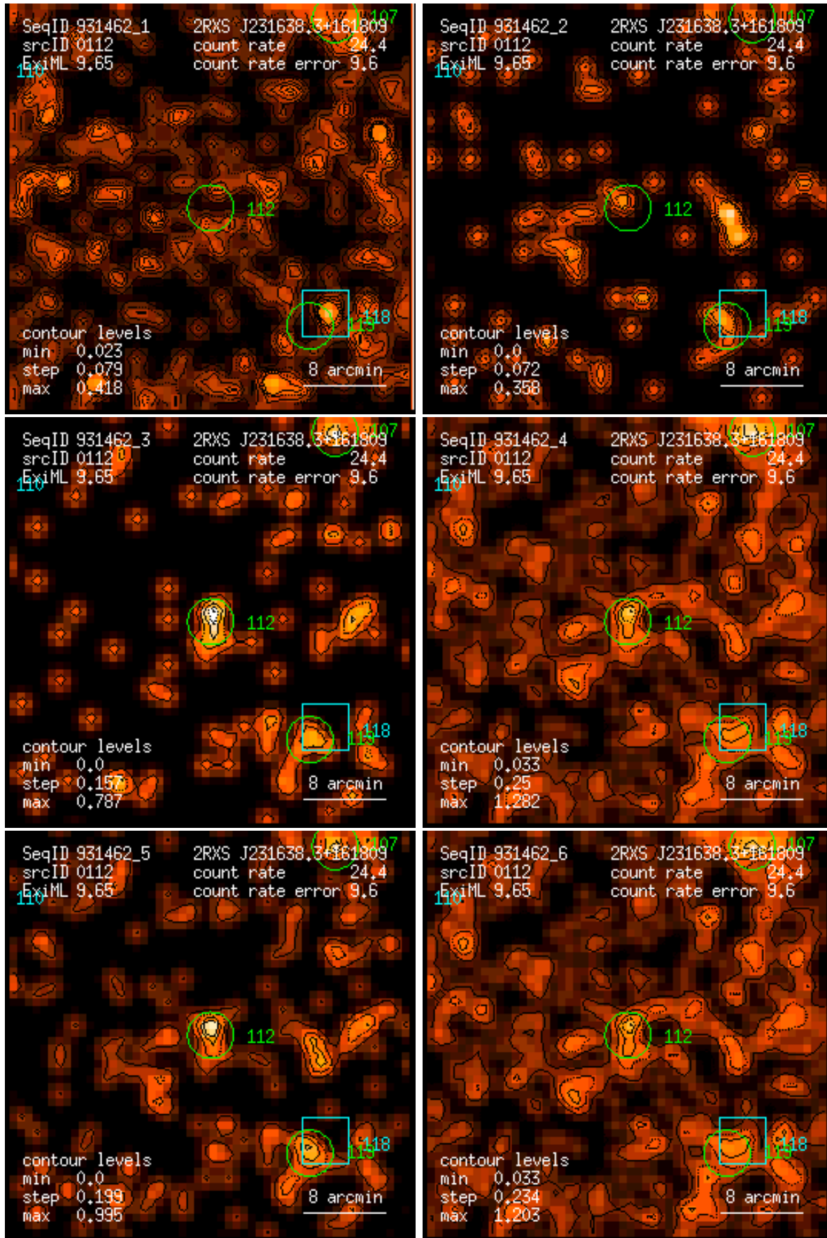
Figure 112: RASS 931462: detection 0112: band rate images, Gaussian filter: (1) PSPC channels 11 – 41, (2) 52 – 90, (3) 91 – 201, (4) 11 – 235, (5) 52 – 201, (6) 11 – 201. Broad band rates in counts/ks. Band rate contour levels in counts/ks/arcmin 2 .
