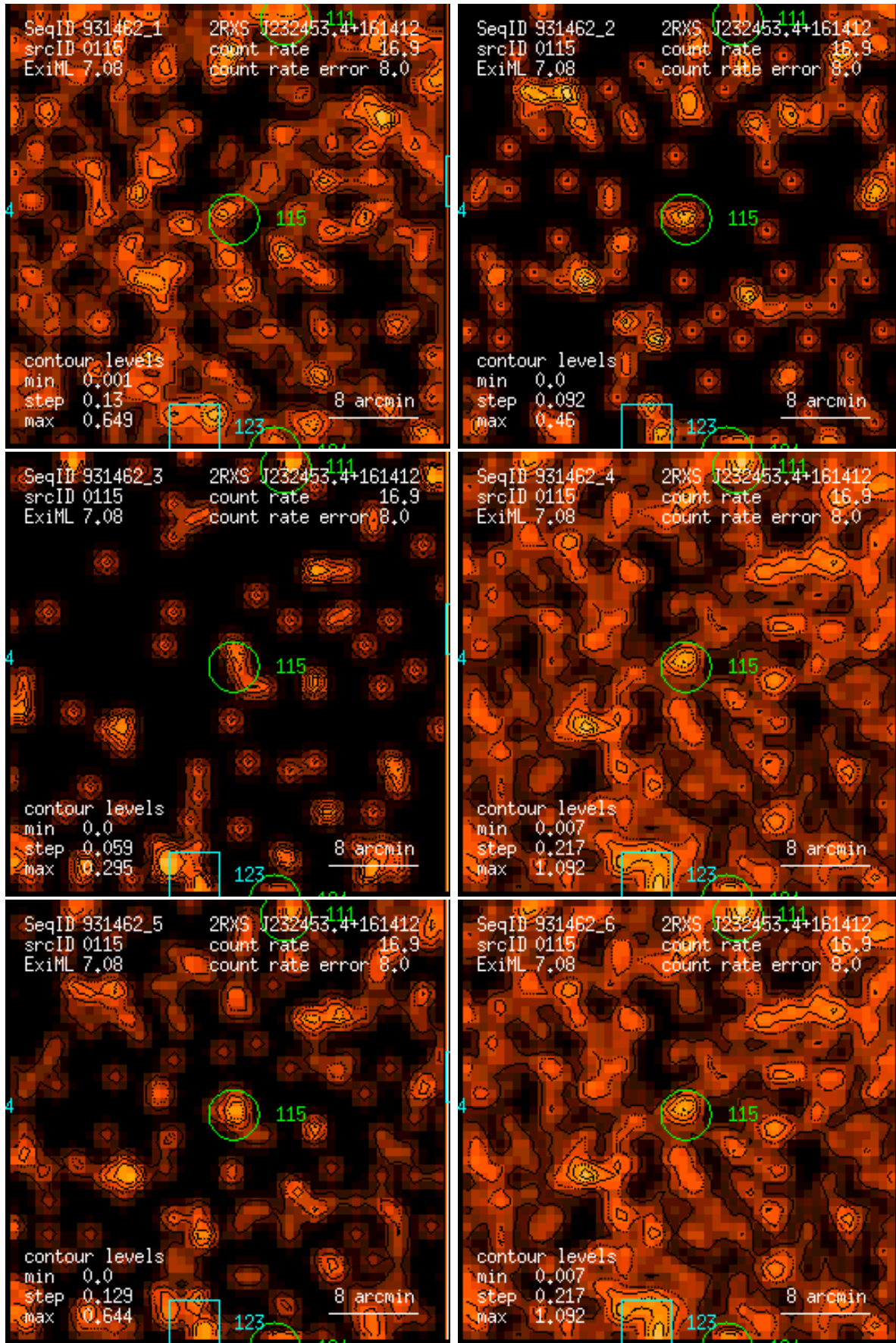
Figure 115: RASS 931462: detection 0115: band rate images, Gaussian filter: (1) PSPC channels 11 – 41, (2) 52 – 90, (3) 91 – 201, (4) 11 – 235, (5) 52 – 201, (6) 11 – 201. Broad band rates in counts/ks. Band rate contour levels in counts/ks/arcmin 2 .
