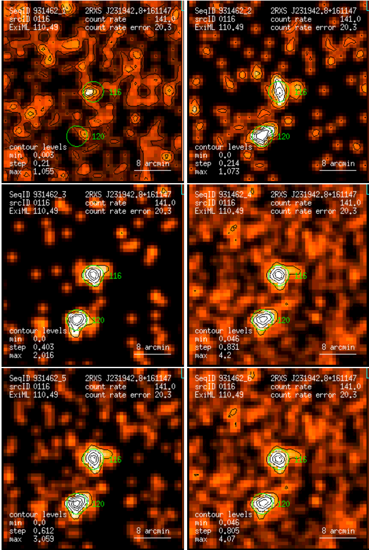
Figure 116: RASS 931462: detection 0116: band rate images, Gaussian filter: (1) PSPC channels 11 – 41, (2) 52 – 90, (3) 91 – 201, (4) 11 – 235, (5) 52 – 201, (6) 11 – 201. Broad band rates in counts/ks. Band rate contour levels in counts/ks/arcmin 2 .
