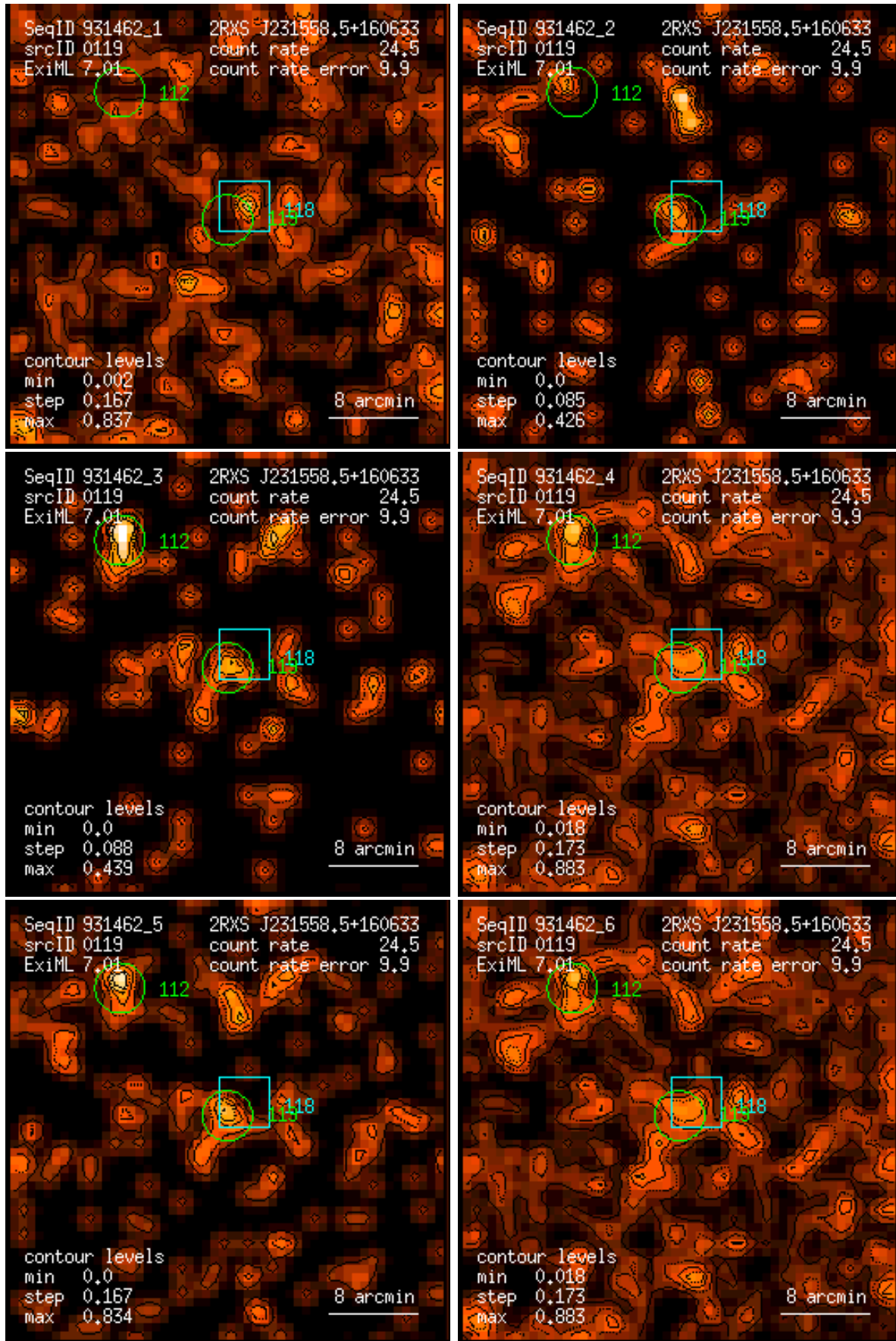
Figure 119: RASS 931462: detection 0119: band rate images, Gaussian filter: (1) PSPC channels 11 – 41, (2) 52 – 90, (3) 91 – 201, (4) 11 – 235, (5) 52 – 201, (6) 11 – 201. Broad band rates in counts/ks. Band rate contour levels in counts/ks/arcmin 2 .
