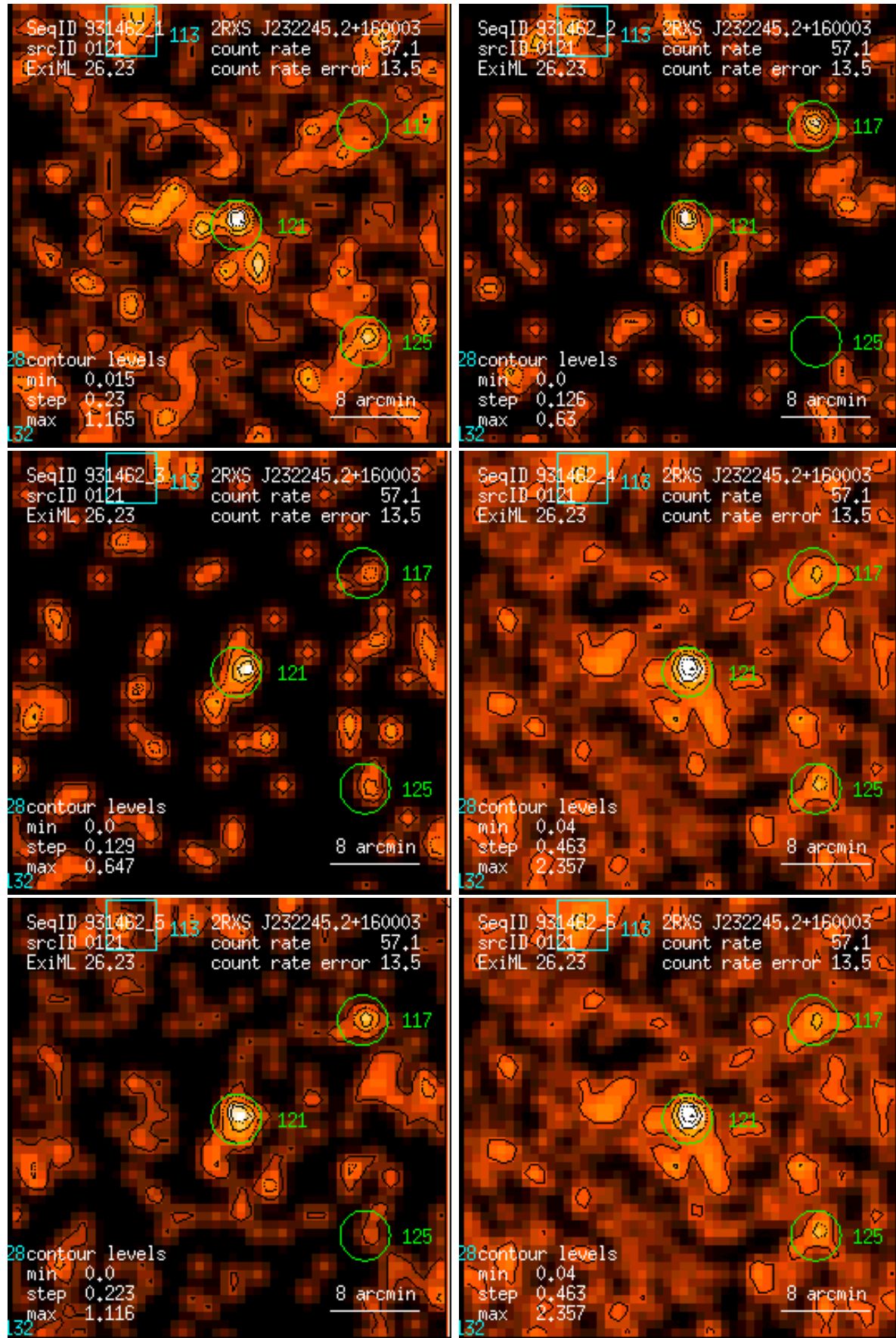
Figure 121: RASS 931462: detection 0121: band rate images, Gaussian filter: (1) PSPC channels 11 – 41, (2) 52 – 90, (3) 91 – 201, (4) 11 – 235, (5) 52 – 201, (6) 11 – 201. Broad band rates in counts/ks. Band rate contour levels in counts/ks/arcmin 2 .
