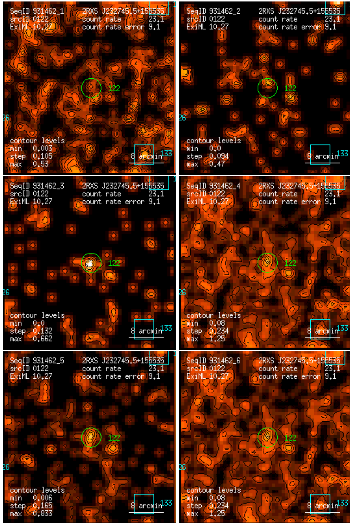
Figure 122: RASS 931462: detection 0122: band rate images, Gaussian filter: (1) PSPC channels 11 – 41, (2) 52 – 90, (3) 91 – 201, (4) 11 – 235, (5) 52 – 201, (6) 11 – 201. Broad band rates in counts/ks. Band rate contour levels in counts/ks/arcmin 2 .
