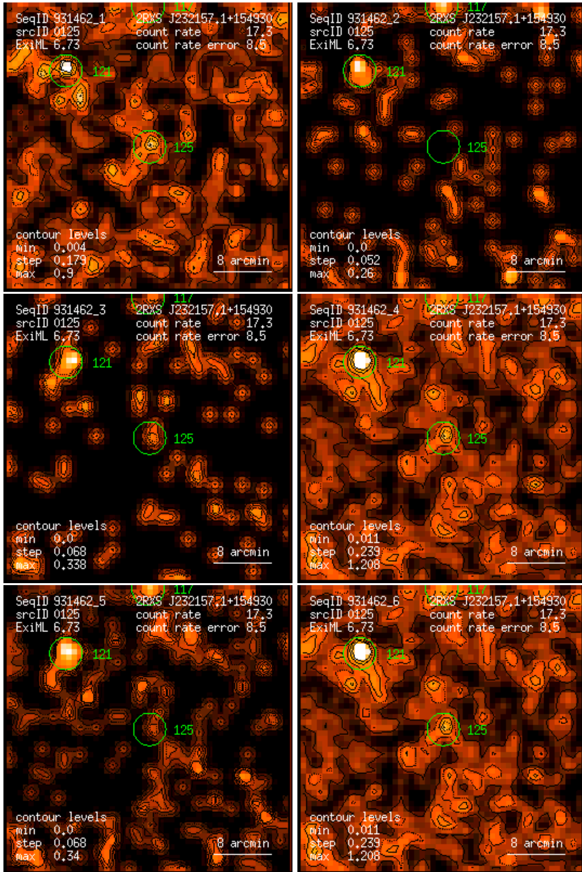
Figure 125: RASS 931462: detection 0125: band rate images, Gaussian filter: (1) PSPC channels 11 – 41, (2) 52 – 90, (3) 91 – 201, (4) 11 – 235, (5) 52 – 201, (6) 11 – 201. Broad band rates in counts/ks. Band rate contour levels in counts/ks/arcmin 2 .
