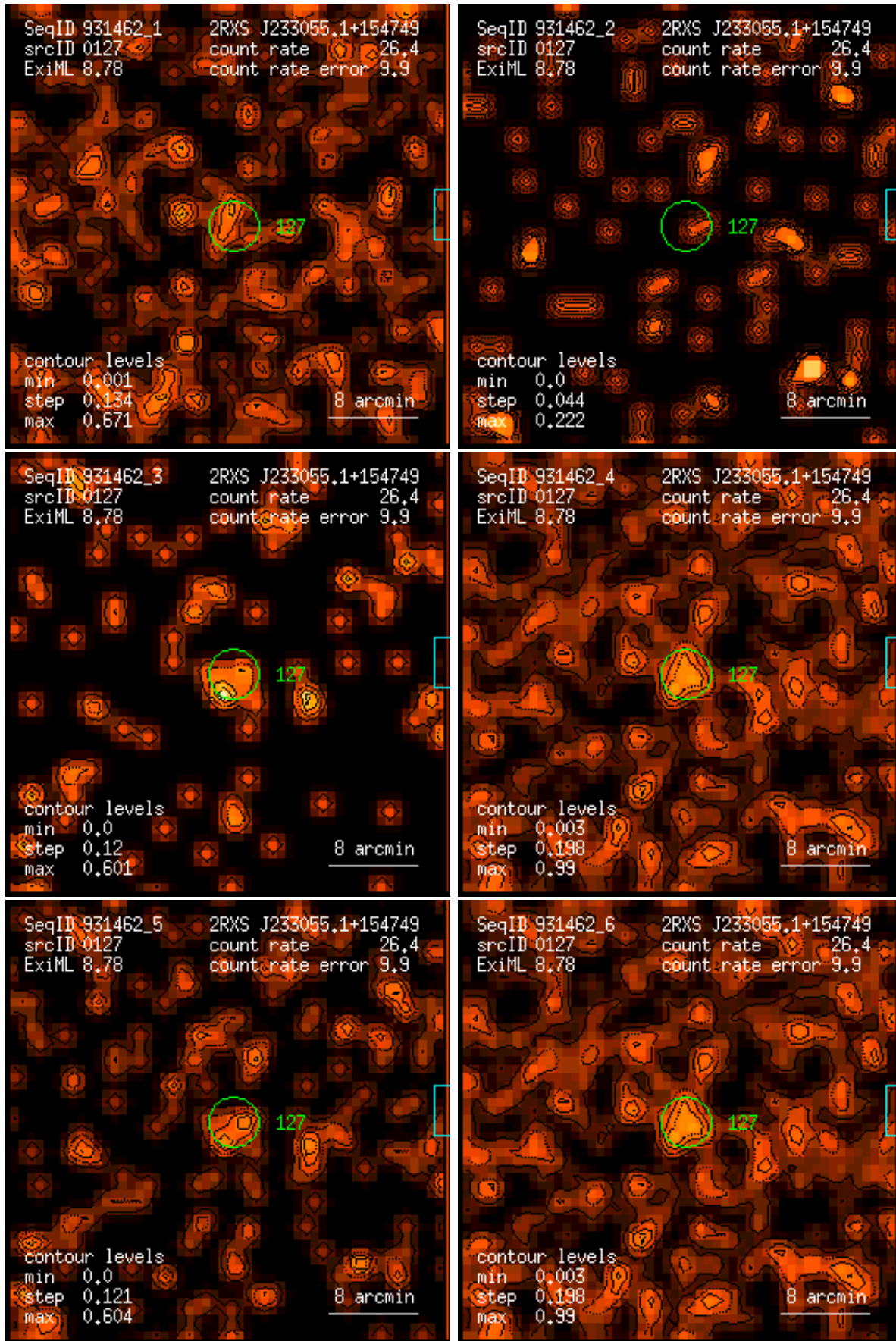
Figure 127: RASS 931462: detection 0127: band rate images, Gaussian filter: (1) PSPC channels 11 – 41, (2) 52 – 90, (3) 91 – 201, (4) 11 – 235, (5) 52 – 201, (6) 11 – 201. Broad band rates in counts/ks. Band rate contour levels in counts/ks/arcmin 2 .
